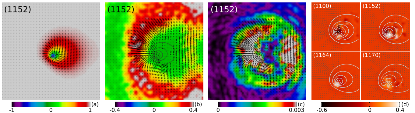
FIG. 3. (Color online) Initial stage of the skyrmion annihilation process [ t = 1152t_0 ; see Fig. 1(b)]: S_z (a), s (b), spin torque |\mathbf{S} \times \mathbf{s}| (c), and electron internal magnetic field b Eq. (10) at different times during the topological transition (d); S_z contour lines (b)–(d); (s_x, s_y) arrows (b)–(d); box size is 64 \times 64a^2 for (a)–(c), and 24 \times 24a^2 for the (d) panel.
