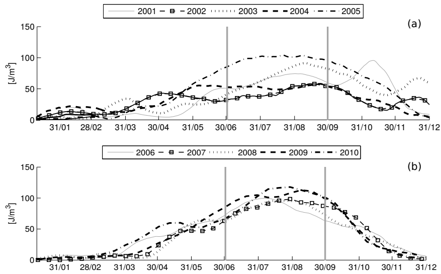
Fig. 3 Time series of 30 day moving averaged potential energy anomaly [Jm^{-3}] over the western part of the GoL for the upper 100 m depth for the years a) 2001 to 2005 and b) 2006 to 2010
