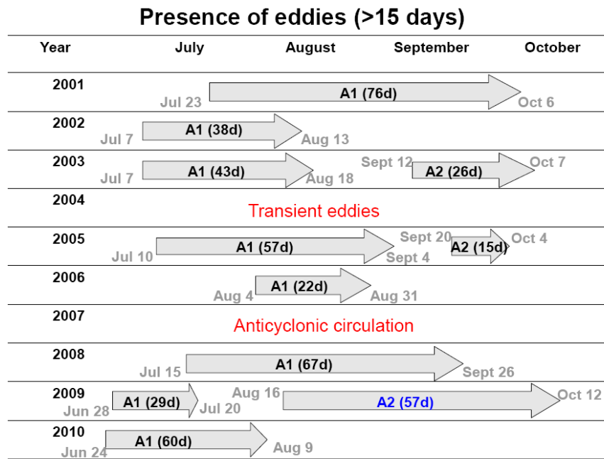
Fig. 5 Gantt table of the long-life modeled eddies from 2001 to 2010. The grey arrows indicate the duration of the first A1 or second A2 eddies, with the corresponding number of days in parenthesis. When this is written in black, the eddy has been generated with the first generation process (Hu et al., 2011b). When in blue, it has been generated by the second generation process (Kersalé et al., 2013). The dates of birth and death of each eddy are also indicated
