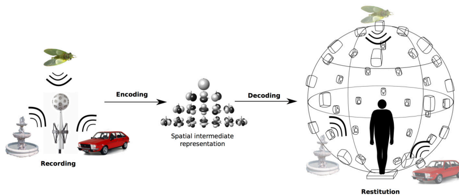
FIGURE 4 | Ambisonics chain. The auditory scene is recorded on the spherical microphone array, encoded in ambisonics, and then decoded on the spherical loudspeaker array to reproduce the whole auditory scene.
