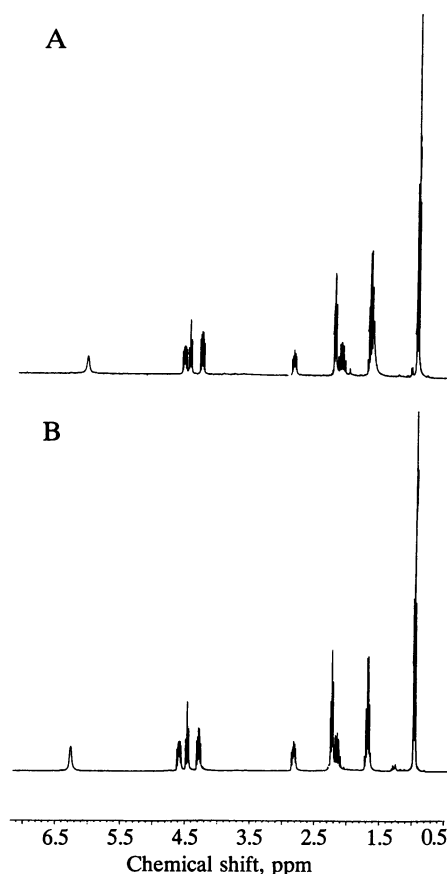
FIG. 3. High-resolution ^1\text{H} NMR spectra of AI-1 purified from spent culture supernatants of E. coli JM109(pMW47.1) (A) and synthetic BHL (B). Spectra were recorded in \text{C}_2\text{H}_2\text{Cl}_3 with tetramethylsilane as the internal standard on a 400-MHz Bruker instrument. The assignment of the signals is as follows: \delta 0.96 (3H, t, J = 7.4 Hz, \text{CH}_3 ), 1.68 (2H, sextet, J = 7.4 Hz, \text{CH}_2\text{CH}_2 ), 2.14 (1H, m, 4\alpha\text{-H} ), 2.24 (2H, t, J = 7.1 Hz, \text{CH}_2\text{CO} ), 2.85 (1H, m, 4\beta\text{-H} ), 4.29 (1H, m, 5\alpha\text{-H} ), 4.47 (1H, td, J = 1.3 and 9 Hz, 5\beta\text{-H} ), 4.56 (1H, m, 3\text{-H} ), 6.06 (1H, br s, NH). The chemical shifts and integrated peak areas of the natural AI-1 and synthetic BHL were indistinguishable.
