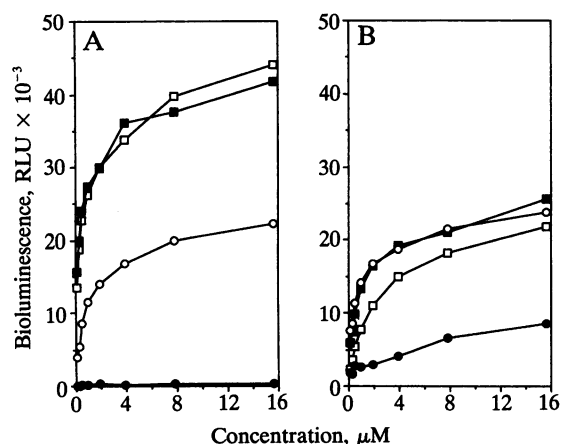
FIG. 5. Dose-response curves for the activity of BHL ( \square ), HHL ( \blacksquare ), OHL ( \circ ), and dDHL ( \bullet ) (A) and their 3-oxo derivatives (B) in the vsmR/vsmI::lux reporter assay. RLU, relative light units.
