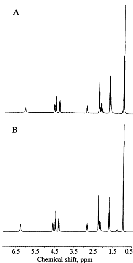
FIG. 3. High-resolution ^1\text{H} NMR spectra of AI-1 purified from spent culture supernatants of E. coli JM109(pMW47.1) (A) and synthetic BHL (B). Spectra were recorded in \text{C}^2\text{HCl}_3 with tetramethylsilane as the internal standard on a 400-MHz Bruker instrument. The assignment of the signals is as follows: \delta 0.96 (3H, t, J = 7.4 Hz, \text{CH}_3 ), 1.68 (2H, sextet, J = 7.4 Hz, \text{CH}_2\text{CH}_2 ), 2.14 (1H, m, 4 \alpha -H), 2.24 (2H, t, J = 7.1 Hz, \text{CH}_2\text{CO} ), 2.85 (1H, m, 4 \beta -H), 4.29 (1H, m, 5 \alpha -H), 4.47 (1H, td, J = 1.3 and 9 Hz, 5 \beta -H), 4.56 (1H, m, 3-H), 6.06 (1H, br s, NH). The chemical shifts and integrated peak areas of the natural AI-1 and synthetic BHL were indistinguishable.
