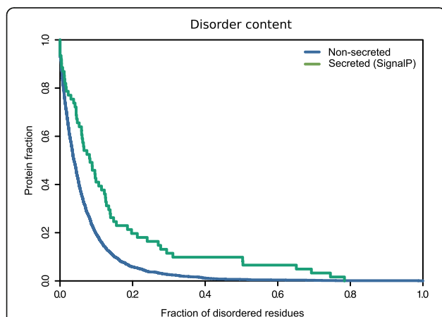
Fig. 2 Disorder propensity of the FusoSecretome . SignalP-secreted proteins show a significantly higher fraction of disordered residues compared to non-secreted proteins ( P value = 1.9 \times 10^{-4} , Kolmogorov–Smirnov test, two-sided)
