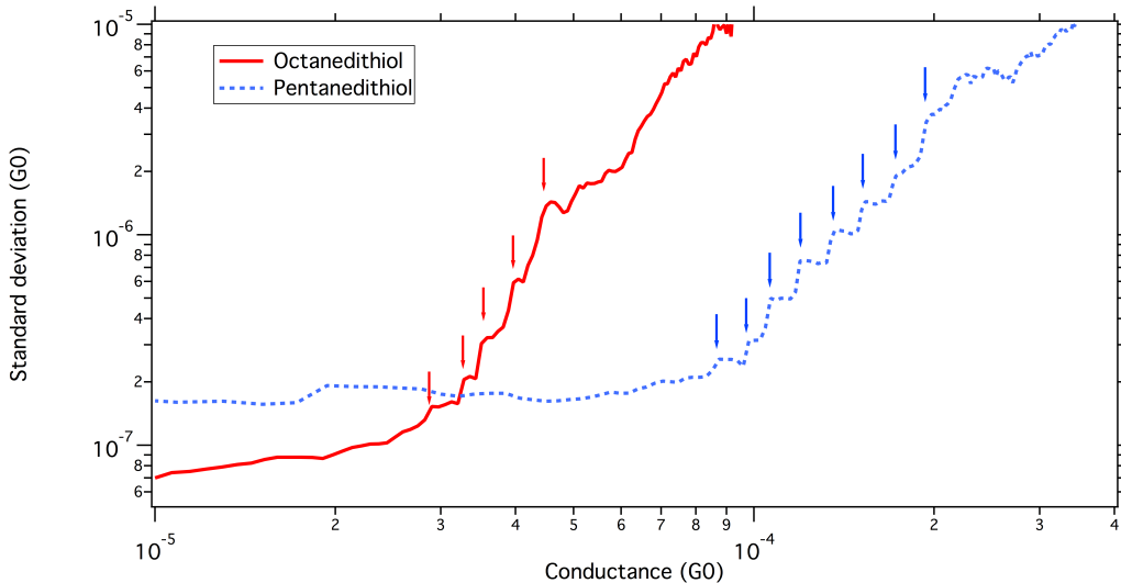
Figure 4: Conductance standard deviation calculated for ODT (continuous line) and PDT (dashed line). Standard deviation data have been binned along the conductance axis (see text for details), and median value of the standard deviation has been calculated for each bin. For both molecules, jumps in the standard deviation appear clearly. The spacing between the jumps along the conductance axis is equal to individual conductance.
