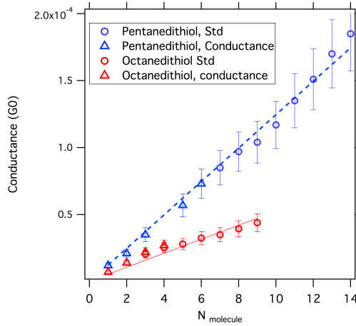
Figure 6: Conductance values corresponding to a discrete number of molecules in PDT and ODT contacts. The plot gathers data extracted from figure 2 and 5. It shows that the conductance values extracted from the two analyses are in excellent agreement. From linear fits we estimate the conductance of a single molecule to be G_{PDT} = 1.25 \cdot 10^{-5} \pm 0.19 \cdot 10^{-5} G_0 for PDT and G_{ODT} = 5.27 \cdot 10^{-6} \pm 0.22 \cdot 10^{-6} G_0 for ODT.
