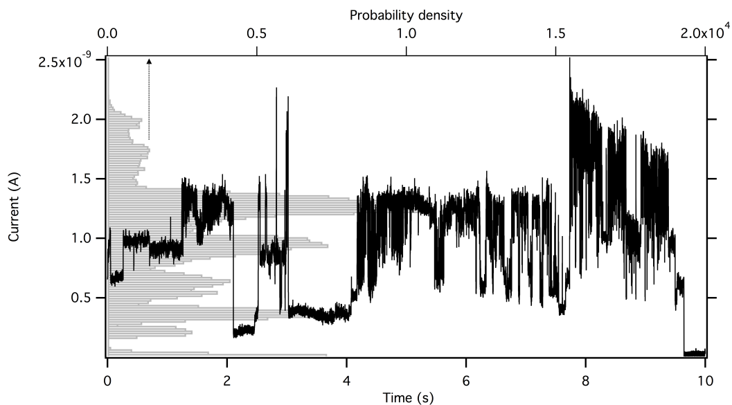
Figure 1: Spontaneous evolution of the current of a molecular contact formed from a millimolar octanedithiol (ODT) solution in mesitylene. Prior to recording, the junction is operated for 2 hours in pure solvent. The recording starts 5 minutes after the junction is refilled with the ODT solution. The electrode separation is fixed with a setpoint current of 0.5nA before the regulation feedback is disabled (see text for more details). Current (black continuous line) is recorded, and a bias of 139mV is applied to the junction. A histogram of the current (gray) clearly indicates the most probable current values.
