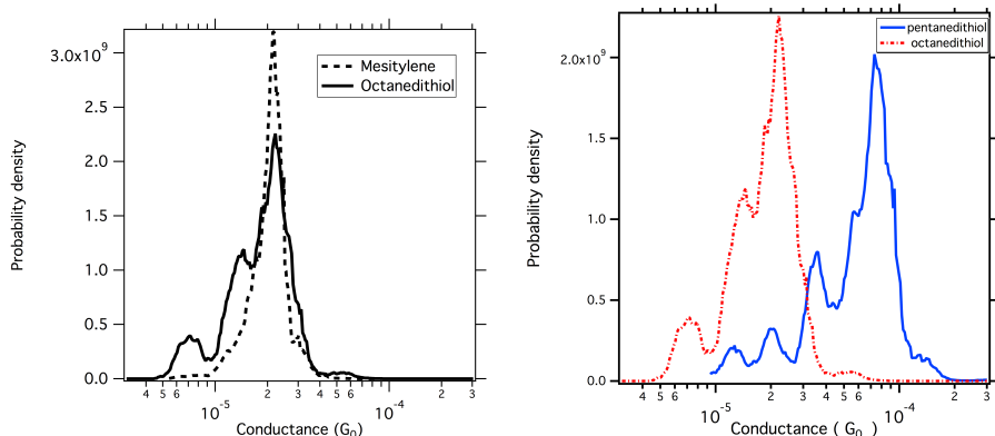
Figure 2: Left : Comparison of conductance histograms for a junction operated in pure mesitylene (black dashed line) and in a millimolar solution of ODT in mesitylene (black continuous line). Bias voltage : 139 mV, setpoint current used to fix the electrode separation : 0.2nA. While the solvent's histogram does not exhibit particular features, it can be seen that a junction containing ODT molecules explores more conductance values and exhibits peaks representing the most probable conductance values. Right : Comparison of conductance histograms for a junction immersed in octane (online version red) and pentanedithiols (online version blue). Bias voltage : 139 mV, setpoint current 0.2nA for octanedithiols and 0.6nA for pentanedithiols. Each histogram exhibits similar features : series of evenly spaced peaks in conductance, which we attribute to the discrete variations in conductance related to the number of molecules in the contact.
