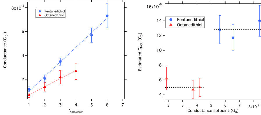
Figure 3: Left : Conductance values of the peaks for the histograms of figure 2 versus a number of molecules. The lower values are attributed to a single molecule as we do not observe current jumps of lower amplitude. A linear fit of these curves gives a conductance per molecule of G_{PDT} = 1.22 \cdot 10^{-5} \pm 5 \cdot 10^{-7} G_0 for PDT, and G_{ODT} = 6.7 \cdot 10^{-6} \pm 4 \cdot 10^{-7} G_0 for ODT. Right : Estimation of conductance values for a single molecule for different conductance setpoints. Bias voltage : 139 mV. The estimated molecular conductance does not depend on the chosen setpoint current.
