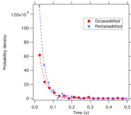
Figure 5: Histogram of the time lag separating conductance jumps for pentane and octanedithiol in mesitylene. The mean time can be interpreted as the lifetime of one molecule in the contact. A fit (lines on plot) with an exponential function A \cdot \exp(-t/\tau) gives equivalent times \tau_{PDT} = 2.6 \cdot 10^{-2} \pm 5 \cdot 10^{-3} s for PDT, and \tau_{ODT} = 3.4 \cdot 10^{-2} \pm 1.3 \cdot 10^{-2} s for ODT.
