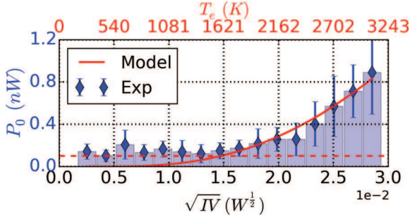
Fig. 4: (Colour online) Experimental (blue columns) and calculated (red continuous line) dependences of the optical power P_0 with \sqrt{IV} . Blue columns correspond to the mean value of the optical power over a binned x -axis. Error bars show the standard deviation calculated over the same binned x -axis. The calculated continuous line allows the determination of the equivalent hot electrons temperature T_e shown on the top x -axis (see discussion section). The dashed horizontal red line represents the noise floor of the optical detector. Data for this figure come from 150 nanojunctions, each of them lasting a few seconds.
