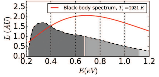
Fig. 5: (Colour online) Calculated emission (red line) and detected (black dashed line) spectra, taking into account the detector spectral response. The black-body temperature is assumed to be 2931 K. Grey scale bands show the spectral bands defined by the semiconductors filters used to gather the integrated optical signal.
