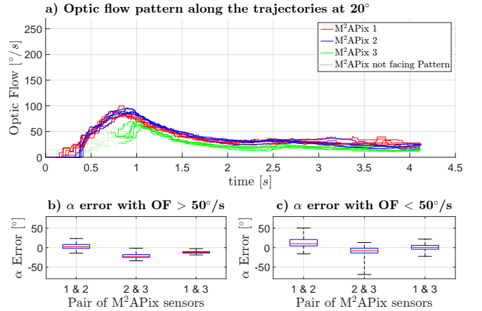
Figure 8: Results obtained on the trajectories at 20°. b) median \pm IQR for pair #1&#2 : 2.0^\circ \pm 10.1^\circ ; for pair #2&#3 : -22.4^\circ \pm 7.6^\circ ; pair #1&#3 : -12.5^\circ \pm 3.7^\circ . c) median \pm IQR for pair #1&#2 : 10^\circ \pm 16.6^\circ ; pair #2&#3 : -7.9^\circ \pm 12.0^\circ ; pair #1&#3 : 0.6^\circ \pm 9.9^\circ .
