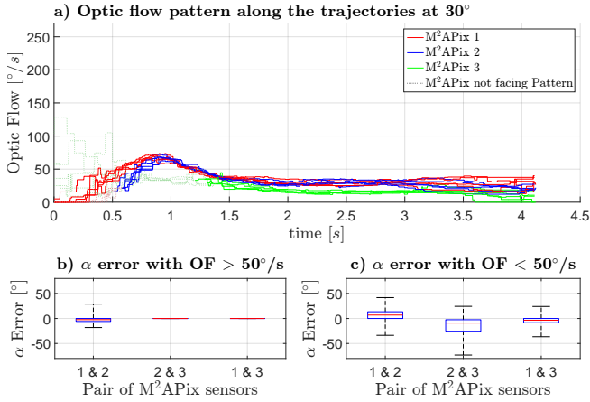
Figure 9: Results obtained on the trajectories 30^\circ . The M^2APix 3 did not measure optic flows greater than 50^\circ/s , which explains the lack of results on the pair of M^2APix #2&#3 and #1&#3 in b). b) median \pm IQR for pair #1&#2 : -2.3^\circ \pm 6.0^\circ . c) median \pm IQR for pair #1&#2 : 6.9^\circ \pm 13.4^\circ ; pair #2&#3 : -9.1^\circ \pm 23.0^\circ ; pair #1&#3 : -3.5^\circ \pm 8.5^\circ .
