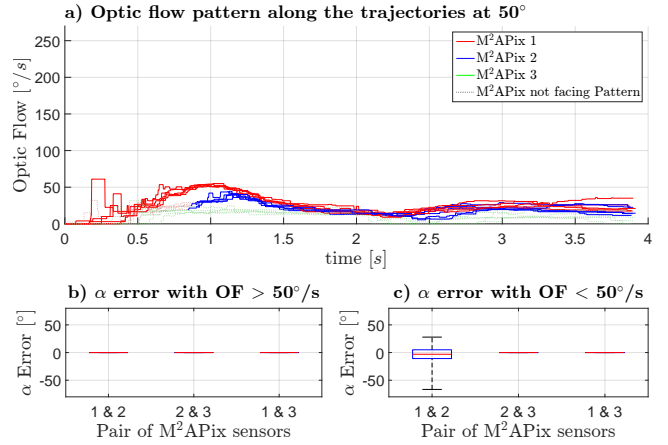
Figure 11: Results obtained on the trajectories at 50^\circ . The pattern on the wall was not visible to M^2APix #3 during all these trajectories, which explains the lack of data on the pair of M^2APix #2&#3 and #1&#3 in c). c) median \pm IQR for pair #1&#2 : -3.1^\circ \pm 15.8^\circ .
