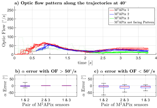
Figure 10: Results obtained on the trajectories 40^\circ . b) median \pm IQR for pair #1&#2 : -2.5^\circ \pm 4.1^\circ . c) median \pm IQR for pair #1&#2 : -3.4^\circ \pm 10.7^\circ ; pair #2&#3 : -7.9^\circ \pm 17.5^\circ ; pair #1&#3 : -6.0^\circ \pm 13.8^\circ .
