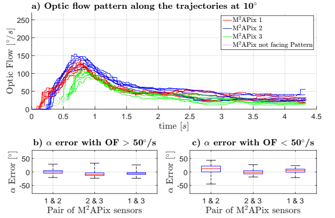
Figure 7: a) Optic flow measurements made by M 2 APix #1 (red), #2 (blue) & #3 (green) during all the trajectories performed at 10°. b) c) Errors distribution of the angles of incidence \alpha recorded per pair of M 2 APix when all the optic flow measurements were greater than 50°/s in b) and less than 50°/s in c), where the red bar is the median, the whiskers correspond to min and max values and the blue box is the IQR at 50%. OF measurements plotted in dotted lines were not generated by the pattern on the wall and were therefore not included in the results presented in b) and c) in this figure and the next ones. b) median \pm IQR for pair #1&#2 : 0.5^\circ \pm 9.6^\circ ; pair #2&#3 : -8.7^\circ \pm 9.8^\circ ; for pair #1&#3 : -5.6^\circ \pm 6.7^\circ . c) median \pm IQR for pair #1&#2 : 12.3^\circ \pm 21.8^\circ ; pair #2&#3 : -1.2^\circ \pm 11.7^\circ ; pair #1&#3 : 5.7^\circ \pm 11.5^\circ .
