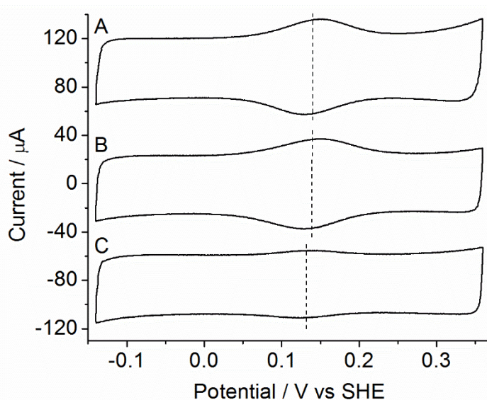
Fig. 4. Cyclic voltammograms of cyt c_{550} (A), cyt c_{550} [C] (B) and cyt c_{550} [N] (C) immobilized on gold NPs modified with mercaptopropionic acid (scan rate 0.1 V. s^{-1} , pH 7).
