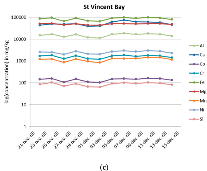
Figure 4. Time variation of the Ca and the 8 metals analysed in SPM trapped during study period from 21 November to 14 December, 2005 in each sampling site: (a) Boulari Bay; (b) Dumbéa Bay and (c) St Vincent Bay.
