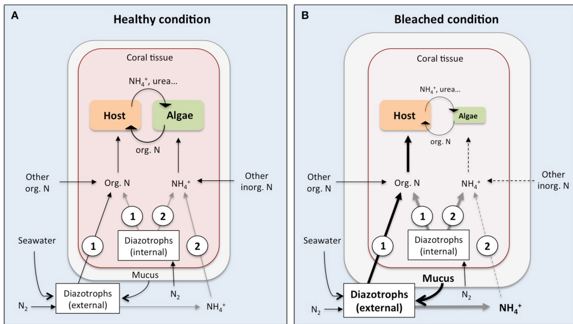
FIGURE 2 | Potential pathways of nitrogen transfer from diazotrophic cells to the coral-zooxanthellae symbiosis under healthy (A) and bleached (B) conditions. The digestion of internal (facultatively associated or symbiotic within the coral tissue) or external (i.e., planktonic or mucus-associated) diazotrophic cells provides organic nitrogen directly to the coral host (1), while fixed nitrogen compounds (in the form of ammonium, \text{NH}_4^+ ) released by internal or external diazotrophs will be primarily available to the zooxanthellae (2). Bold arrows indicate potential amplification of pathways in bleached corals, where an increased diazotrophic abundance in the mucus layer combined with increased heterotrophic feeding on bacterial cells may provide additional nitrogen to the coral host. This could outbalance the reduced ability of corals to take up dissolved inorganic nitrogen from the surrounding seawater under thermal stress and bleached conditions (dashed lines). Black arrows indicate known pathways while gray arrows represent potential pathways that have not been empirically demonstrated yet.
