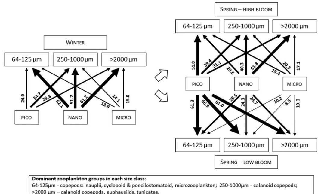
Figure 8. Relative contributions picoplankton, nanoplankton, and microplankton biomass to the biomass of three zooplankton size fractions in the Liguro-Provençal Basin in WINTER and SpringHB and SpringLB based on isotope mixing model outputs (see section 2 and Figure 7). Arrows indicate the transfer of material between pico-POM, nano-POM, and micro-POM fractions and zooplankton size classes, and their thickness is proportional to relative contribution. Values of percentage contributions determined from the mixing model are located against the corresponding arrow. Winter was a period of low phytoplankton biomass across all size fractions; SpringHB is representative of the deep convection zone in the central basin with high nutrients and high phytoplankton biomass dominated by nanophytoplankton and microphytoplankton; and SpringLB is representative of the region outside the convection zone dominated by nanophytoplankton. Zooplankton size classes: 64–125 μm—copepods: nauplii, cyclopoid, and poecilostomatoid; 250–1000 μm—calanoid: copepods; >2000 μm—calanoid: copepods, euphausiids, tunicates, gelatinous predators, and amphipods.
