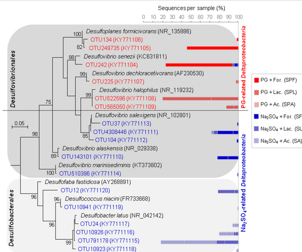
FIGURE 5 | Maximum-likelihood (ML) tree based on 16S rRNA gene sequences showing the phylogenetic position of Deltaproteobacteria enriched from marine sediment (as inoculum) using different electron donors and sulfate sources (sodium sulfate or phosphogypsum). Representative sequences in the tree were obtained from GenBank (accession number in the brackets). Bootstrap values >75% are indicated at nodes. The bars represent the relative abundance of each OTU affiliated with Deltaproteobacteria in the enrichment cultures. The blue bars indicate the relative abundance of OTUs in sodium sulfate cultures, whereas the red bars represent the relative abundance of OTUs in PG cultures.
