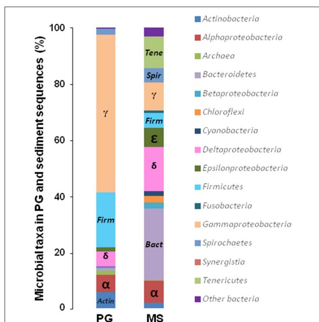
FIGURE 1 | Compositions of microbial communities in the coastal marine sediment and phosphogypsum samples of Sfax (Tunisia). Relative phylogenetic abundance was based on frequencies of 16S rRNA gene sequences affiliated with Archaea and major bacterial phyla or proteobacterial classes in the microbial communities of marine sediment (MS) and phosphogypsum (PG).
