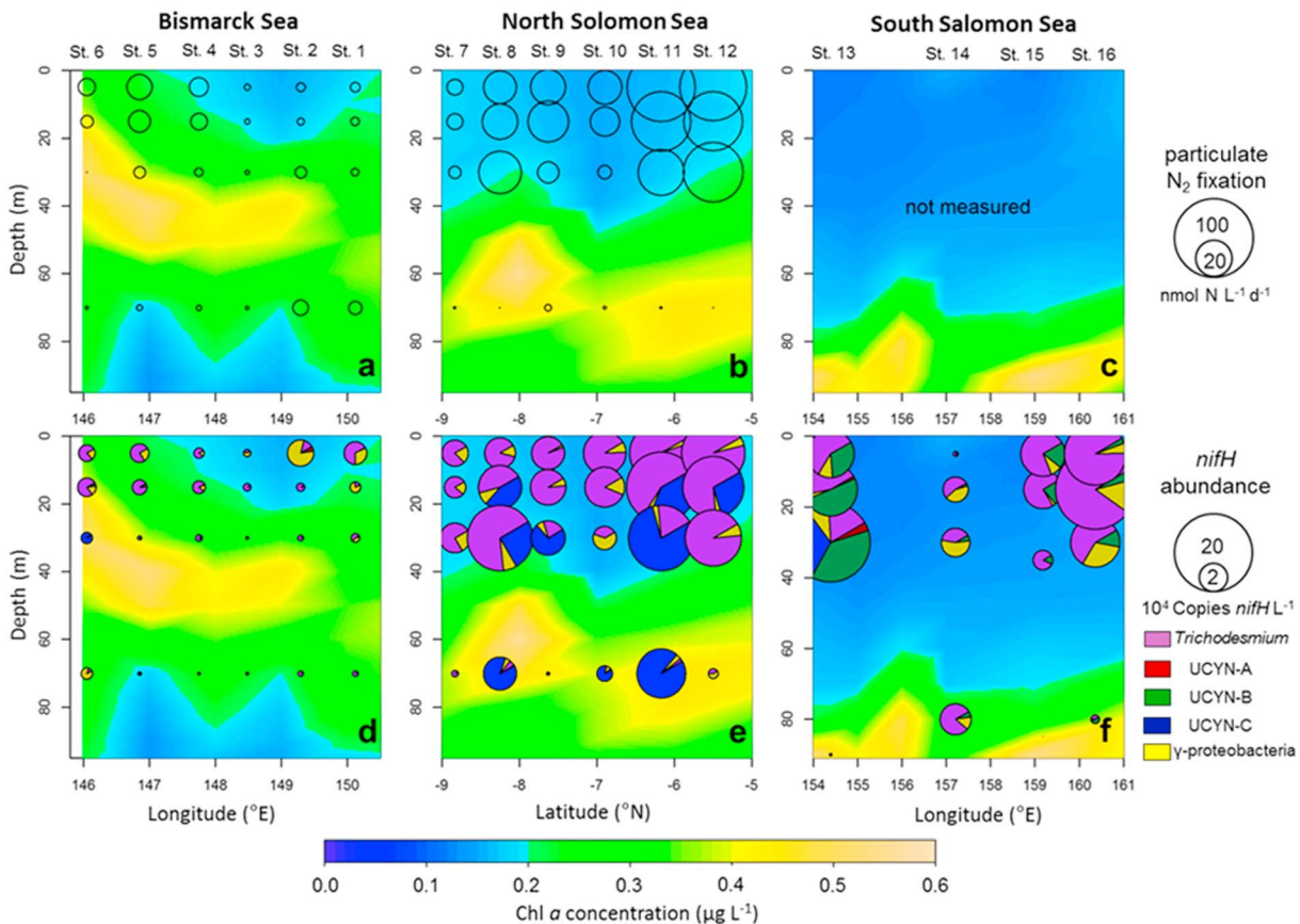
Figure 1. Vertical and horizontal distribution of the PN 2 fixation rates are shown in nmol N L -1 d -1 in the (a) Bismarck Sea, (b) North Solomon Sea, and (c) South Solomon Sea. Vertical and horizontal distribution of the nifH gene abundances in copies L -1 (sized dots) in the (d) Bismarck Sea, (e) North Solomon Sea, and (f) South Solomon Sea. Colors indicate the proportion of Trichodesmium (purple), UCYN-A (red), UCYN-B (green), UCYN-C (blue), and γ-24774A11 Gammaproteobacterium (yellow). DDAs abundances were several orders of magnitude lower than the other diazotrophs and hence are not shown. The color scale refers to Chl a concentrations in µg L -1 .
