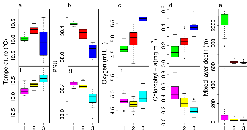
Figure 3. Boxplot of temperature, salinity, oxygen and chlorophyll- a within the upper 250 m of the water column, and depth of the mixed layer, for (top) (a–e) L1 and L2 (bottom) (f–j) following clusters defined in Figure 2 (same colors).
