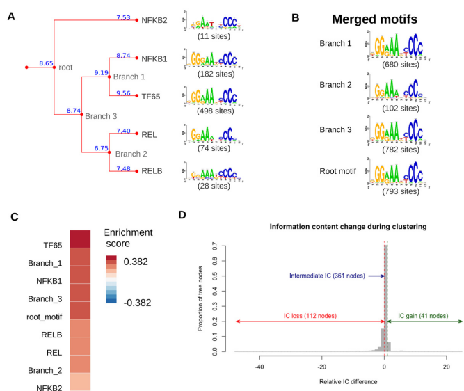
Figure 6. Information content and predictive power of the unclustered and clustered motifs. (A) Clustering of five HOCOMOCO human motifs bound by NF- \kappa B-related factors. The blue numbers at the tree branches indicate the information content of each PSSM. The number of sites used to build each matrix is indicated in parenthesis. (B) Logos of the merged motif at each level of the tree. (C) Enrichment of predicted NFKB binding sites for original and merged (branch + root) motifs in ChIP-seq peaks for RelA in Hodgkin Lymphoma Cell Line (GEO entry GSM1556331) (64). (D) Distribution of IC relative differences measured during the clustering of 519 human TFBMs from HOCOMOCO.
