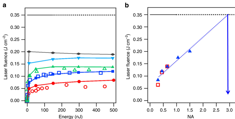
Fig. 2 Maximum delivered laser fluences inside silicon with ultrashort pulses. Measurements ( hollow symbols ) and simulations ( solid symbols ) for evaluating the peak fluence delivered with 60-fs laser pulses focused at a depth of 1 mm inside silicon. a Dependence on the incoming laser pulse energy evaluated for increasing numerical apertures (NA): NA = 0.3 (red), NA = 0.45 (dark blue), NA = 0.65 (green), NA = 1 (light blue), and NA = 1.5 (gray). b Fluence saturation levels plotted as a function of NA. Taken as a target, the dark horizontal line is the measured threshold for modification with the same laser beam at the surface of the sample. The blue arrow indicates by extrapolation that a NA near 3 is required to cross this fluence threshold in the bulk
