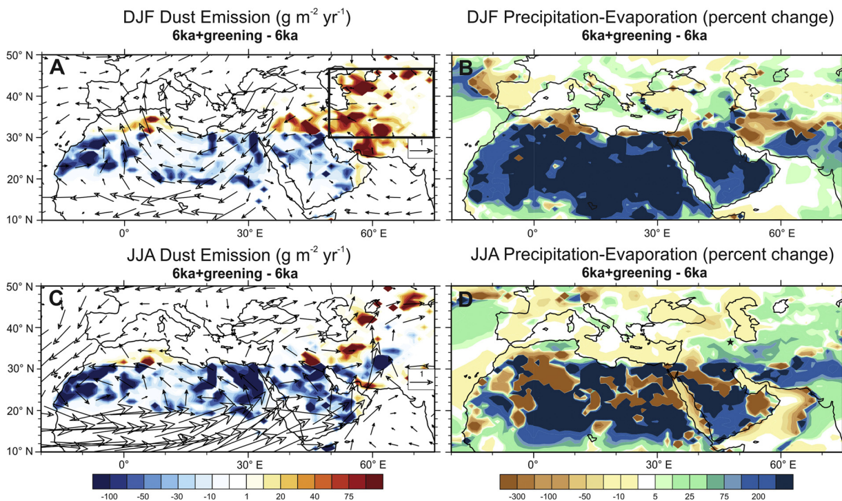
Fig. 10. Boreal winter (DJF) and summer (JJA) dust emission anomalies and 800-hPa wind vector anomalies and precipitation minus evaporation. Boreal winter (A) and summer (C) dust emission anomalies (6 ka + greening – 6 ka) in \text{g m}^{-2} \text{ yr}^{-1} . Wind vector anomalies at 800 hPa are overlaid with a reference vector length of 1 \text{ m s}^{-1} . Black star denotes the location of the study site. Boreal winter (B) and summer (D) precipitation minus evaporation anomalies (given as a percent change). The dark gray box in panel A shows the location of the West Asian box used to calculate the seasonal and annual mean dust emission anomalies. (For interpretation of the references to color bar in this figure, the reader is referred to the web version of this article.)
