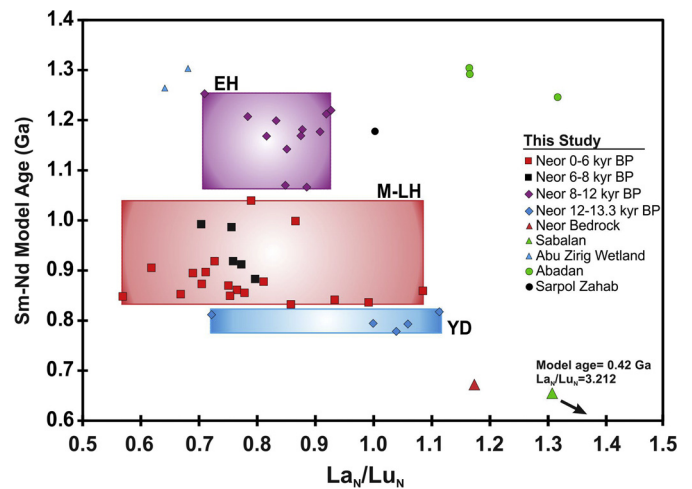
Fig. 7. Difference in Sm–Nd model ages compare to normalized La_N/Lu_N ratios. Colored boxed represent clusters of Neor paleo-dust samples for the Younger Dryas (YD), the early Holocene (EH) and the mid-late Holocene (M–LH). Colors and symbols are same as in Fig. 3. (For interpretation of the references to color in this figure legend, the reader is referred to the web version of this article.)
