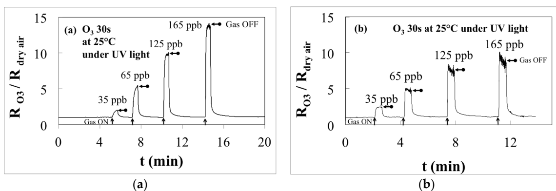
Figure 2. Normalized responses at 25 °C for O_3 sensors based on ZnO at 30 mg/mL (post-annealed at 80 °C) under UV light (a) without EA (S1) and (b) with EA (S2).
