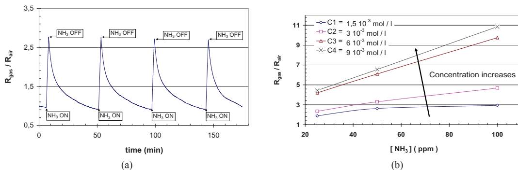
Figure 3: (a) Repetitive sensor response under 100 ppm \text{NH}_3 . (b) Sensitivity Evolution according to four concentrations of DH-DS2T solution.
