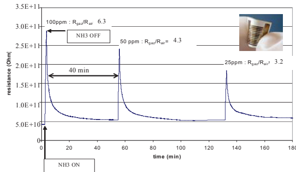
Figure 2: Ammonia sensor response of a sensor based on DH-DS2T drop casted layer on flexible PET substrate ( \text{NH}_3 exposition time = 2 min). R_{\text{gas}}/R_{\text{air}} : normalised response defined as the sensor resistance ratio ( R_{\text{gas}} ) to that in synthetic dry air ( R_{\text{air}} ).
