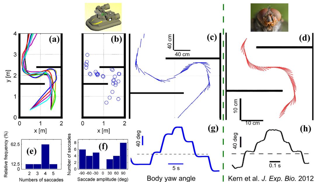
Fig. 9. Direct comparison between the behaviour of the simulated robot and that of the blowfly in an S-shaped turn. (a) 8 simulated robots trajectories in a challenging corridor comprising an S-shaped turn 0.80 m in width, starting at an initial position ( x_0 = 0.5 m; y_0 = 0.35 m) with various initial orientations \Psi_0 = (35^\circ; 40^\circ; 45^\circ; 50^\circ) , or an initial position ( x_0 = 1.5 m; y_0 = 0.35 m) and various initial orientations \Psi_0 = (70^\circ; 80^\circ; 90^\circ; 95^\circ) . (b) Points in the corridor at which the saccades occurred. (c) Typical trajectory of the robot among the set of 8 trajectories presented in (a). The position of the robot (black circles) and its body orientation (blue lines) are plotted every 400 ms. (d) Typical trajectory of a blowfly in an S-shaped turn, adapted from data published by (Kern et al., 2012). Position of the fly (black circles) and its long body axis (red lines) are plotted every 10 ms. Inset: head of a Calliphoravomitioria (Picture: J. J. Harrison, Wikimedia commons). (e) Relative frequency of saccades per trajectory while navigating the S-shaped turn ( n = 30 ). (f) Body saccades were classified depending on their amplitude: -90^\circ , between -89^\circ and -60^\circ , between -59^\circ and -30^\circ , then between 30^\circ and 59^\circ , between 60^\circ and 89^\circ , and 90^\circ . (g) Robot's body yaw angle during the trajectory shown in (c). The horizontal dashed line gives the corridor's y-axis ( \Psi = 90^\circ ). (h) Fly's body yaw angle during the trajectory shown in (d). The horizontal dashed line indicates the tunnel y-axis ( \Psi = 90^\circ ). Data adapted from (Kern et al., 2012). From Serres and Ruffier (2015). ©Elsevier. (For interpretation of the references to colour in this figure legend, the reader is referred to the web version of this article).
