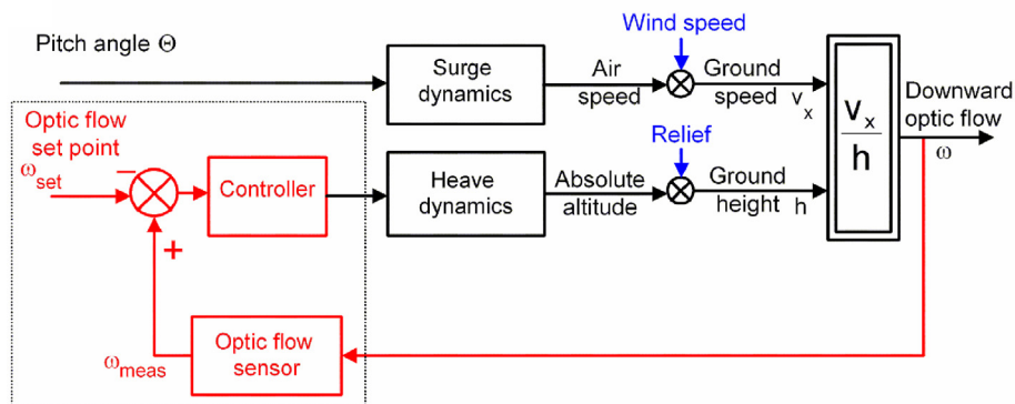
Fig. 13. OCTAVE autopilot based on a ventral optic flow regulator (OCTAVE stands for Optic flow based ConTrol system for Aerial VEHICLES). The optic flow regulator controls the lift at all times so as to maintain the downward optic flow constant despite wind and relief disturbances. From Franceschini et al. (2007). ©Elsevier.
