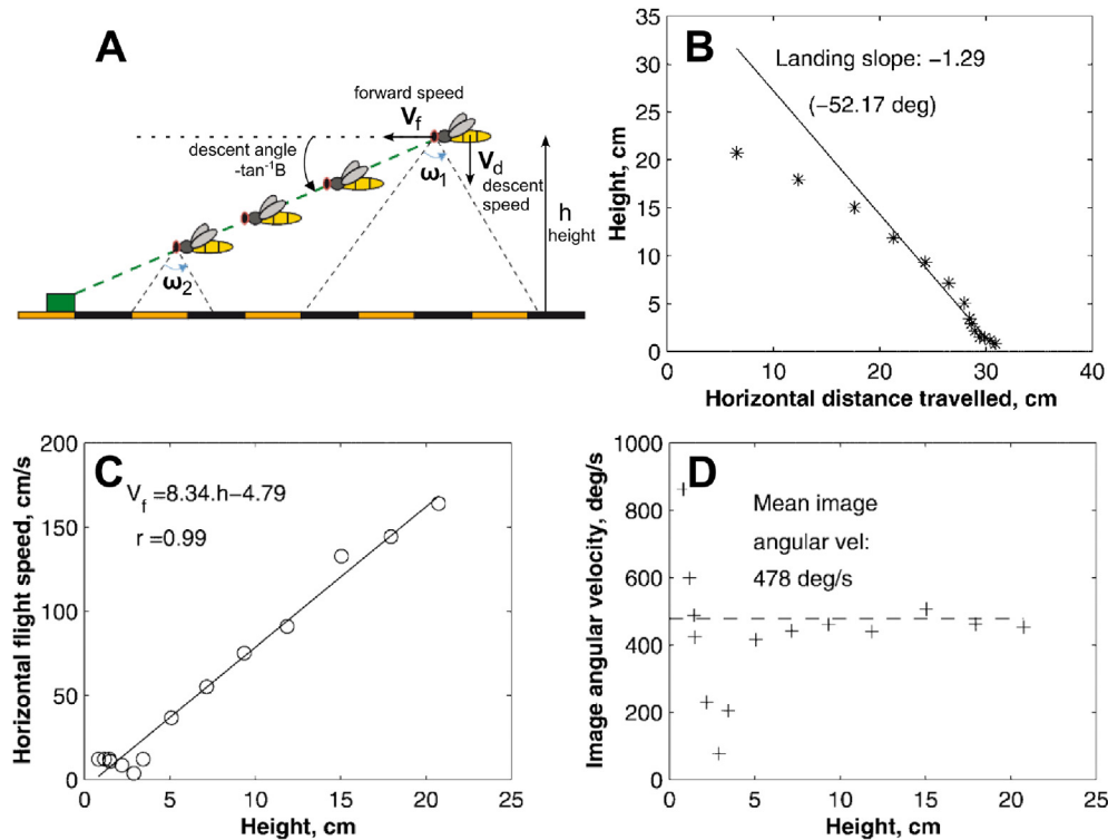
Fig. 11. (A) Parameters during a bee landing: h flight height, V_f forward speed, v_d descent speed, \tan^{-1} B descent angle, \omega_1 and \omega_2 the optic flow for two distinct positions. Adapted from Srinivasan (2011). (B) Bee trajectory along the vertical plane with a descent angle of -52^\circ (Srinivasan et al., 2000) ©Springer. (C) Forward speed V_f as a function of the height h showing a strong correlation between these two flight parameters (Srinivasan et al., 2000) ©Springer. (D) The ventral optic flow is maintained constant at about 478^\circ/\text{s} during the bee's landing (Srinivasan et al., 2000) ©Springer.
