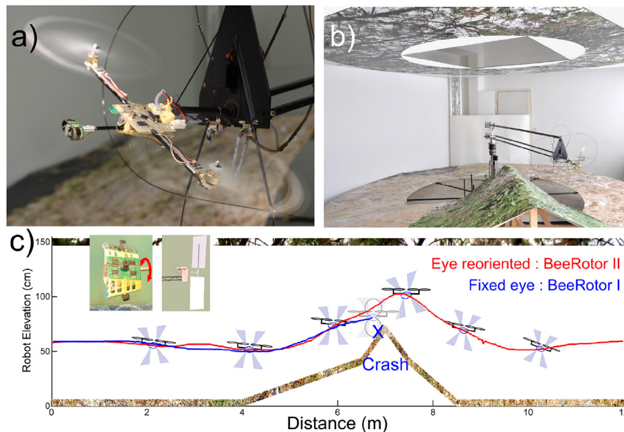
Fig. 14. (a) BeeRotor I robot equipped with the full cylindrical CurACE sensor (Floreato et al., 2013). (b) Photograph of the experimental set-up. (c) Trajectories of the robot BeeRotor II that automatically follows the ground, thanks to the ventral optic flow regulator and the fixed eye (blue) and decoupled eye (red) oriented parallel to the ground. This reorientation enables the robot, at an earlier stage, to detect the increase in the optic flow due to steep relief. Adapted from Expert and Ruffier (2015) under CC-BY license. (For interpretation of the references to colour in this figure legend, the reader is referred to the web version of this article).
