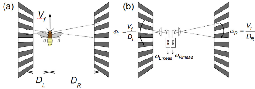
Fig. 6. (a) The right \omega_R and left optic flow \omega_L perceived by a bee flying in the horizontal plane along a corridor at a forward speed V_f . The bee is at a right clearance D_R and a left clearance D_L from the walls, and \omega_R and \omega_L are angular velocities at which two opposite points in the wall texture placed directly at a right angle seem to move. (b) By definition, \omega_R and \omega_L (in rad/s) are the ratios between the forward speed and the distance from the walls. A minimalistic “pair of sensitive optic flow neurons” is used inside the bee’s brain: each one comprises a lens and two photoreceptors driving an Elementary Motion Detector (EMD). Each output, \omega_{Rmeas} and \omega_{Lmeas} , serves as feedback signals to jointly control the flight speed and lateral position.
