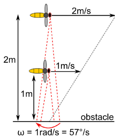
Fig. 2. The chicken-and-egg problem of the translational optic flow. An infinite number of couples (speed; distance) lead to the same speed/distance ratio, so the same angular velocity (optic flow magnitude). For instance in this picture an optic flow value of 1 \text{ rad/s} (or 57^\circ/\text{s} ).
