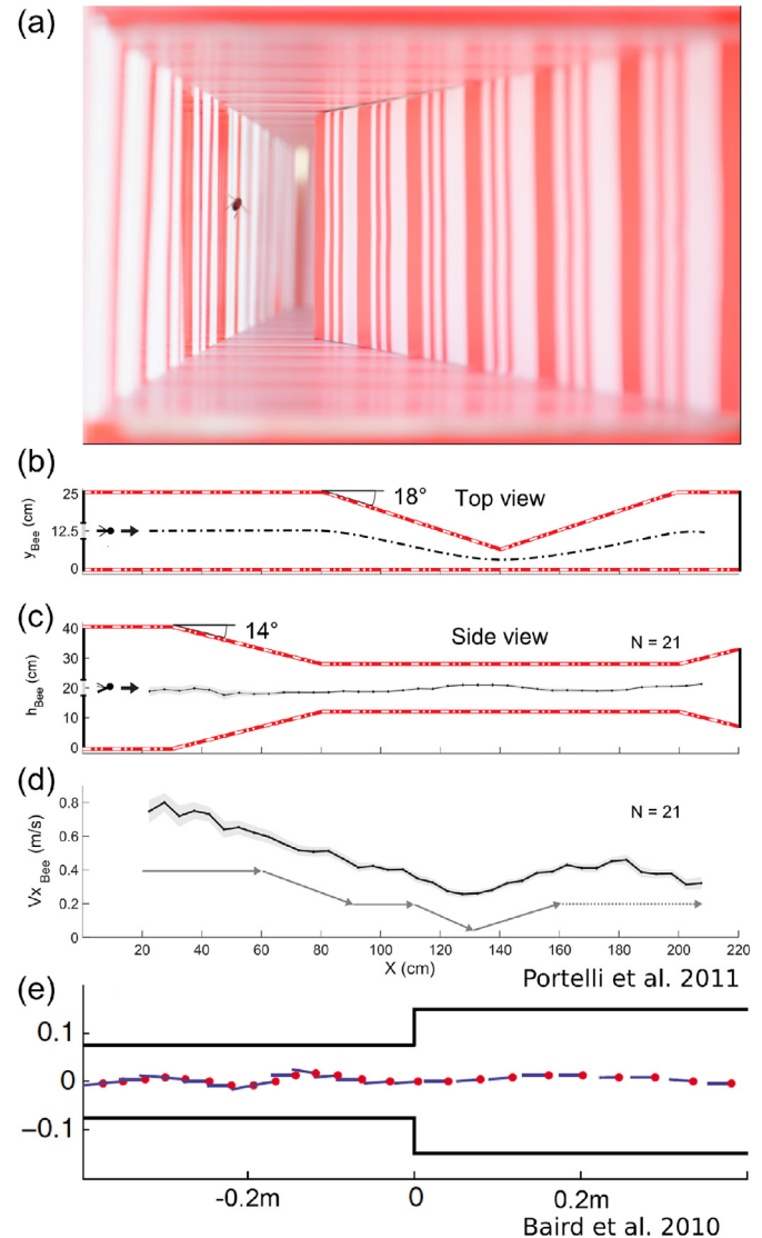
Fig. 3. (a) A honeybee flying along the doubly-tapered tunnel. The photograph was taken from the entrance of the tunnel. ©DGA/F. Vrignaux. (b) Top view of the tunnel showing the honeybee's entrance, the part tapering in the horizontal plane and the guessed trajectory of the bee in the horizontal plane with respect to the "centring response". (c) Side view of the tapered tunnel, showing the vertical constriction. The mean flight path of the honeybees is plotted as a function of the distance along the abscissa. The bees' mean trajectory can be seen to be practically vertically centered throughout the tunnel (height h = 19 \pm 0.16 \text{ cm} ). (d) Ground speed profile along the tunnel. The honeybees decreased their speed as the tunnel narrowed and increased their speed as it widened. The faded trace around the curves gives \pm the standard error of the mean. The gray profile underneath the main curve shows the overall flight speed pattern as shown by the analysis. Adapted from Portelli et al. (2011). (e) The honeybees flew at low speed as the tunnel was narrow and increased their speed as it widened abruptly. Adapted from Baird et al. (2010).
