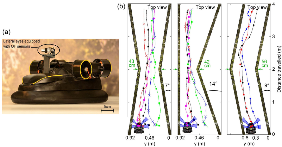
Fig. 7. (a) A fully autonomous sighted hovercraft equipped with a minimalistic (8-pixel) compound eye. (b) Automatic wall-following behaviour as a function of the initial ordinate in both tapered and bent corridors. From Roubieu et al. (2014) under CC-BY License.
