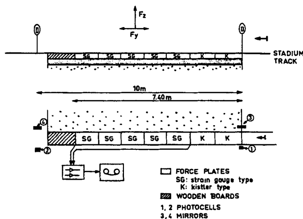
Fig. 1. Schematic description of the force platform and time-measuring device (photocells).
