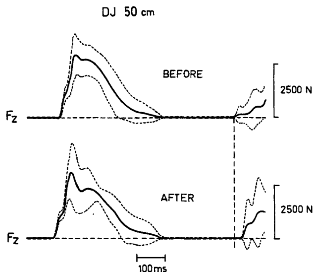
Fig. 10. Group-averaged (mean \pm SD) F_z curves of the before and after marathon drop-jump test.
