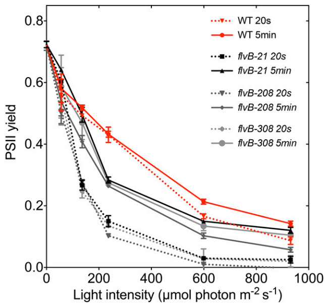
Figure 3. Light dependence of the PSII yield in the wild type (WT) and flvB mutant strains. Upon 10-min dark adaptation under constant air bubbling, algal suspensions of wild type and flvB mutant strains were introduced in the cuvette of a pulse amplitude-modulated fluorimeter. PSII yields were measured after 20 s (dotted lines) or 5 min (plain lines) of illumination at different light intensities. Shown are the mean values ( \pm SD, n = 3 ).
