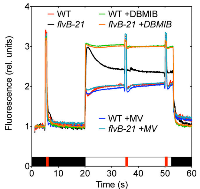
Figure 4. Effect of DBMIB and MV on chlorophyll fluorescence transients measured in wild type (WT) and flvB mutant strains. Samples were placed in the dark (black box) in the presence of 1 \mu\text{M} DBMIB, 1 \text{ mM} MV, or without addition of any chemicals. Chlorophyll fluorescence was measured during a transient dark to light ( 100 \mu\text{mol photon m}^{-2} \text{s}^{-1} ) transient. Saturating flashes were supplied when indicated by red vertical lines. Shown are the traces representative of n = 2 independent measurements. Fluorescence data have been normalized on F_0 .
