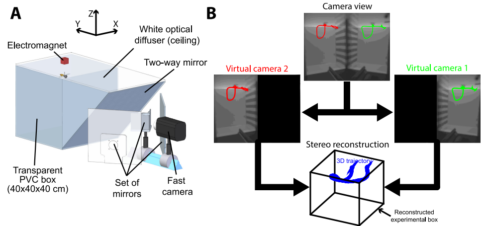
Fig 3. Setup and stereo reconstruction. (A) The setup consists of a 40 \times 40 \times 40 \text{ cm}^3 box illuminated from above with a halogen light. Hoverflies were filmed in the box with a fast camera through a two-way mirror at a rate of 1600 frames per second in full resolution (1280 by 800 pixels). The mirror was tilted at an angle of 45^\circ to make the hoverfly see a uniform white wall (i.e. the reflection of the white light-diffusing ceiling). A manual switch was used to trigger the camera and simultaneously turn off the power of the electromagnet, thus releasing the resting fly and causing it to fall. A set of mirrors was used to split the images, giving two different views of the experimental box. (B) Example of a split image obtained with the set of mirror with the two trajectories superimposed. The two trajectories were used to obtain a 3-D reconstruction with the MATLAB stereo vision toolbox.
