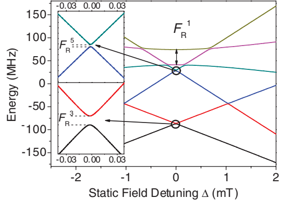
FIG. 4. (Color online) Dressed-state energies for H_0 \parallel [100] , h_{\text{MW}} = 0.8 mT, and m_I = 1/2 . The large anticrossing F_R^1 is the one-photon Rabi splitting. The insets are close-ups of the three-photon and five-photon Rabi splittings.
