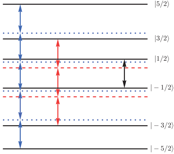
FIG. 1. (Color online) Level diagram of the \text{Mn}^{2+} spin in a cubic crystal field for a Zeeman splitting \gamma H_0 = E_{1/2} - E_{-1/2} . Arrows indicate one-photon (black), three-photon (red), and five-photon (blue) monochromatic transitions between spin projections m , as shown on the left-hand side. The dashed and dotted lines show equidistant virtual levels enhancing the multiphoton transitions.
