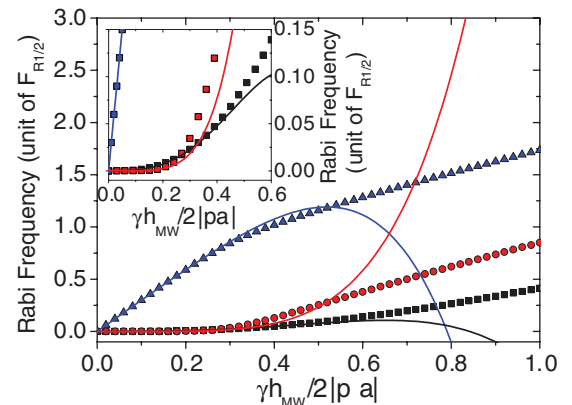
FIG. 9. (Color online) Rabi frequency dependence as a function of the reduced MW field \tilde{h} . Data points are numerically computed by solving Eq. (A1), while lines are the analytical perturbation developments [Eqs. (A3)–(A5)]. The inset shows a close-up at low fields and low Rabi frequencies.
