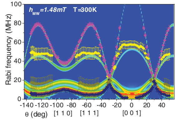
FIG. 6. (Color online) Rabi frequency distribution of \text{MgO:Mn}^{2+} while the static field H_0 rotates in the plane (-110) and for a microwave field h_{\text{MW}} = 1.48 mT. The static field H_0 = 348.5 mT and frequency f = 9.676 GHz are set to probe the transition |m_S = -1/2, m_I = 1/2\rangle \leftrightarrow |m_S = 1/2, m_I = 1/2\rangle . The points represent peaks in the Fourier transform of the experimental data. The error bars are the width of the Fourier transform (consequence of the damping). The color plot is calculated with the numerical model given in Sec. IV B.
