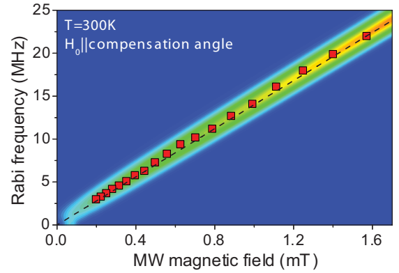
FIG. 8. (Color online) Rabi frequencies as FFT peaks (solid squares) of coherent oscillations for H_0 along the compensation direction of the cubic anisotropy \theta = \theta_{\text{CA}} . The color plot is numerically computed, as described in Sec. IV B, while the dashed line shows the expected behavior for an isotropic S = 5/2 system [see Eq. (A7)].
