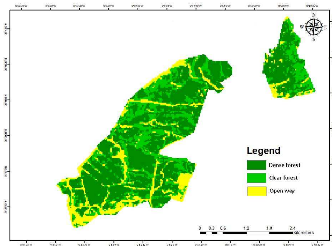
Fig. 2: Image classification Landsat 5 TM since 2014(t2)
