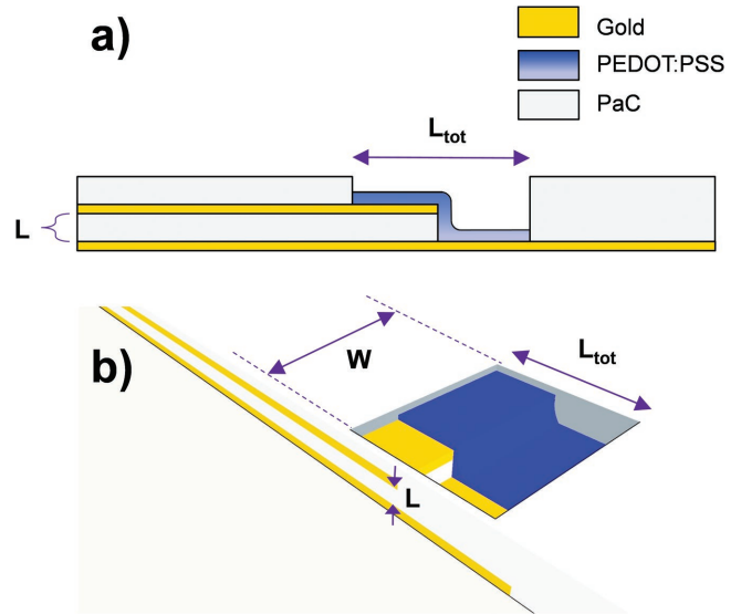
Figure 1. vOECT structure. a) Cross-sectional view demonstrating how the PaC layer thickness defines the channel length ( L ). b) Top view with PEDOT:PSS shown partially filled in, to aide in the visualization of L . W and L_{\text{tot}} are defined by the PaC opening, L_{\text{tot}} is specified for calculation of the total PEDOT:PSS layer volume.
