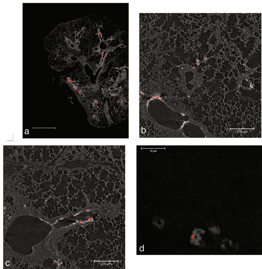
Figure 4. 2D slices virtually extracted from reconstructed 3D images, a grayscale colormap is used. Segmented pixels are colored in red. (a) LFOV scan, 1 px = 14.32 \mu\text{m} , scale bar = 1000 \mu\text{m} (b,c) HRes scan, 1 px = 1.09 \mu\text{m} , scale bar = 200 \mu\text{m} (d) nano-CT scan, 1 px = 63.5 nm, scale bar = 10 \mu\text{m} .
