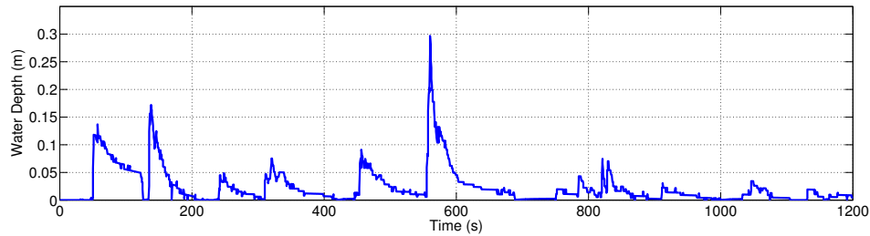
Figure 9: Time series of water depth measured to the SW of Oléron Island (France) on the 08/02/2016, showing overshoot associated with IG waves with periods ranging from 70 to 100 s. Adapted from Baumann et al. (2017).
