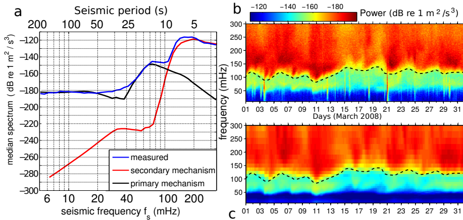
Figure 15: Measured and modeled seismic spectra. (a) Vertical acceleration power spectral density (PSD) in March 2008 at the French SSB seismic station, located near Saint-Etienne, France. (b) observed and (c) modeled PSDs in March 2008 following Hasselmann (1963) and Arduin et al. (2015). Light blue to red vertical stripes correspond to earthquakes (not modeled). The dashed line separates the low frequencies where the primary mechanism dominates from the higher frequencies explained by the secondary or 'double-frequency' mechanism. The Johanna storm, on March 10, is conspicuous with powerful and lower frequency microseisms.
