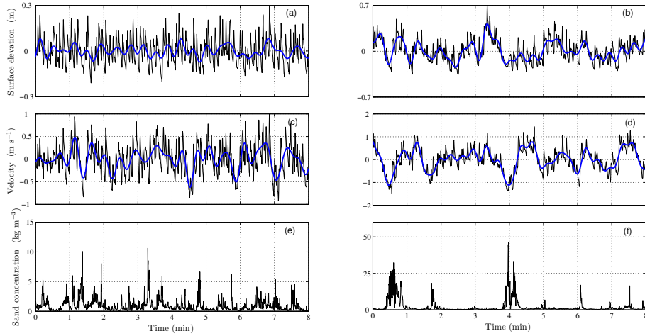
Figure 10: Example timeseries of a positive correlation r_0 (a,c,e) in the inner-surf zone of the steeply sloping Zandmotor beach and a negative r_0 (b,d,f) in the inner-surf zone of the gently sloping Ameland beach. Please note the different y-axis scales. (a,b) sea-surface elevation (m) and (c,d) cross-shore velocity with in black the total velocity, and in blue the IG velocity, and (e,f) sand concentration. For Ameland location P11, h = 1.00 m, r_0 = -0.04 , H_{total}/h = 0.67 , \bar{u} = -0.15 m/s, H_{IG}/H_{SW} = 1.00 . For the Zandmotor location P10, h = 0.5 m, r_0 = 0.17 , H_{total}/h = 0.66 , \bar{u} = -0.16 m/s, H_{IG}/H_{SW} = 0.39 . After De Bakker et al. (2016).
