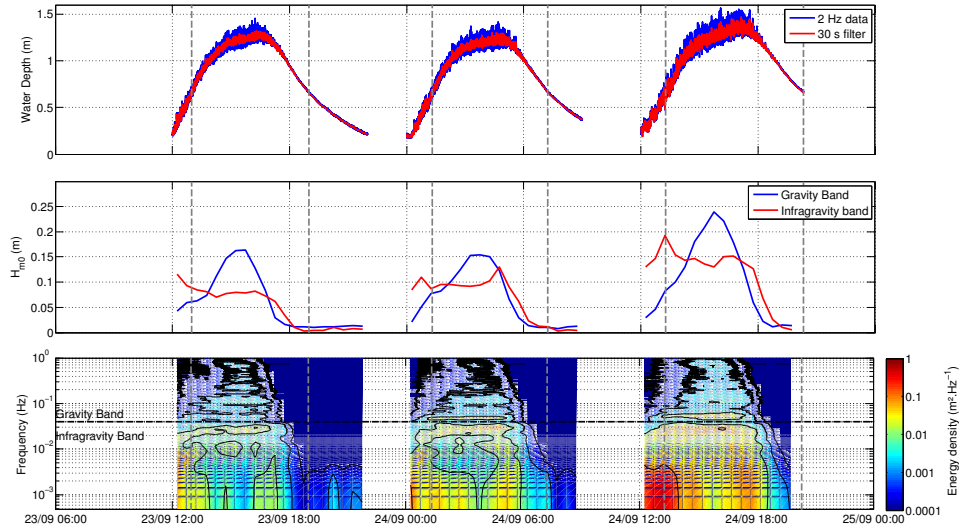
Figure 12: Time-series of observed water depths (top), H_{m0} in the gravity (blue) and in the (red) IG bands (middle) and frequency repartition of the energy density inside the Albufeira Lagoon (Portugal) in September 2010
