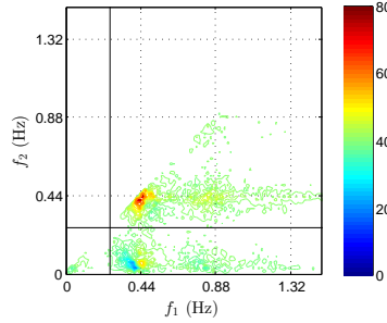
Figure 17: Imaginary part of the bispectrum in m^3 ( \times 10^{-8} ) of the incoming wave signal ( \eta^+ ) over a 1:80 laboratory slope, at x = 70 m, h = 0.18 m. Black solid lines indicate the cutoff between infragravity and sea-swell wave frequencies, f_{IG} . Dashed lines indicate the spectral peak ( f = 0.44 Hz) and its higher harmonics. After De Bakker et al. (2015a).
