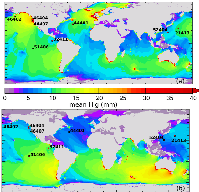
Figure 16: Mean values of H_{IG} over (a) January and February 2008, (b) June and July 2008. Small square with numbers correspond to the location of DART stations used here for model validation. Taken from Ardhuin et al. (2014).
