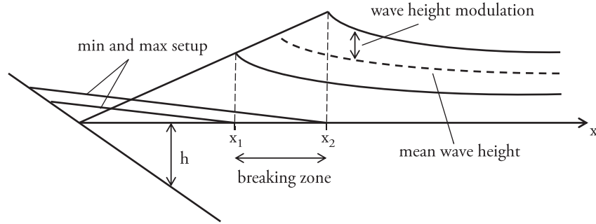
Figure 3: Schematic representation of the cross-shore variation of the minimum, mean and maximum short wave height, with the associated steady state setup through the surf zone. x_1 and x_2 are the minimum and maximum positions of the breakpoint, and h is the water depth. (Figure reproduced from Symonds et al. (1982).)
