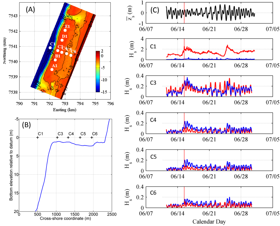
Figure 13: (A) Bathymetry of Ningaloo Reef (Western Australia) and location of the sensors, (B) cross-shore profile of the reef at the location of the sensors and (C) Time series of the mean water level (tide) measured on the forereef at C1 and Root-mean-square wave heights for the IG wave band H_{rms,IG} (blue) and short-wave band H_{rms,sw} (red) measured across at C1, C3, C4, C5 and C6). Modified from Van Dongeren et al. (2013)
