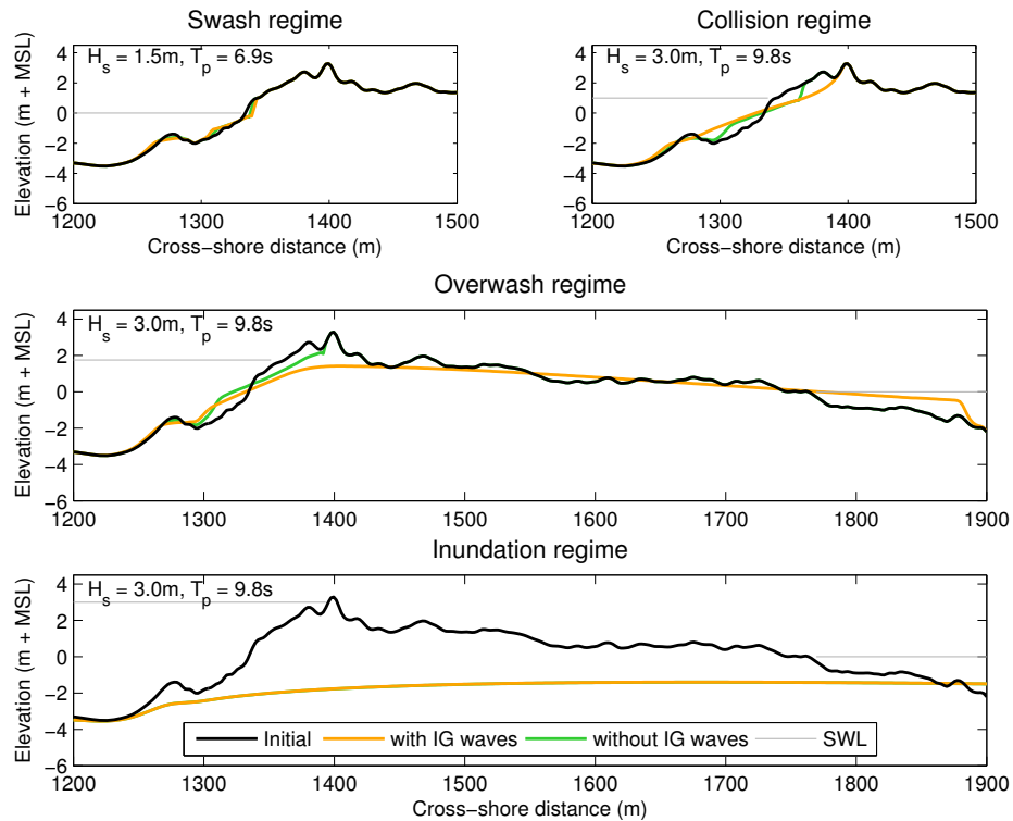
Figure 11: Simulated morphological change of a cross-shore profile of a barrier island based on McCall et al. (2010) using the XBeach model with (orange) and without (green) IG waves. Four simulations are run in which the barrier island is exposed to four different water level, wave height and wave period forcing conditions for a duration of three hours to characterise storms in the swash, collision, overwash and inundation regimes, as defined by Sallenger (2000). Differences between the models are particularly apparent in the collision and overwash regime.
