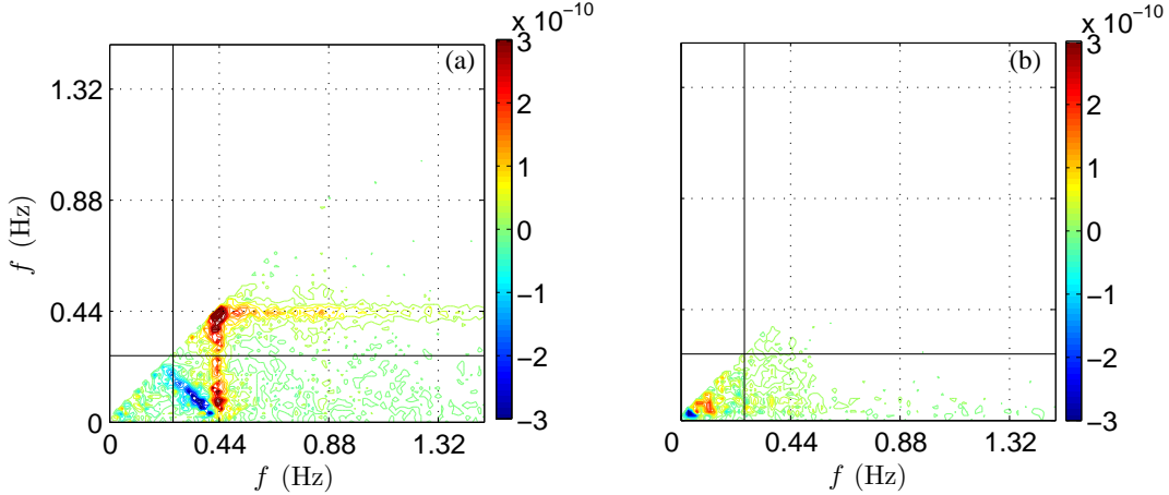
Figure 5: Imaginary part of the bispectrum in m^3 ( \times 10^{-6} ) of the incoming wave signal ( \eta^+ ) for a narrow-banded wave condition over (a) a 1:20 slope and (b) a 1:50 slope in a water depth h of 5 cm (equal to h = 1 m in the field) for values where b^2 > b_{95\%} . Dashed lines indicate the spectral peak ( f = 0.44 Hz) and its higher harmonics and the solid lines correspond to the frequency cutoff between IG waves and short waves. After: De Bakker et al. (2015b)
