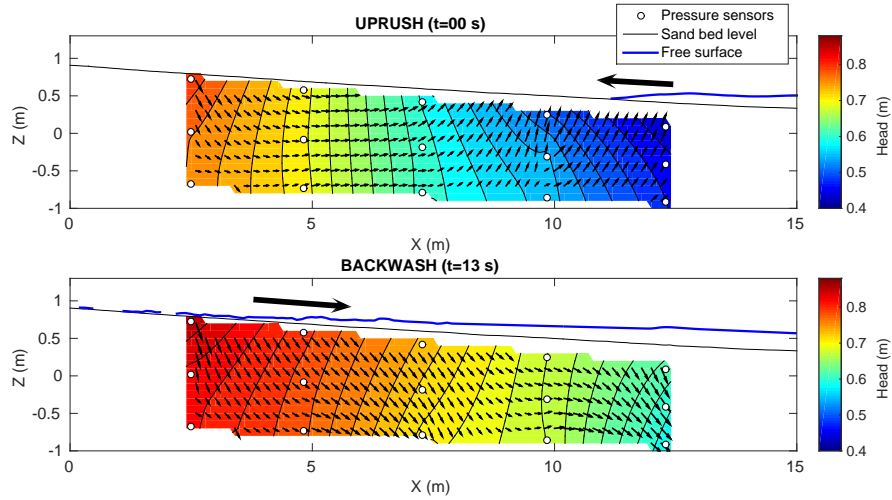
Figure 8: Groundwater pressure head and velocity fields during uprush (top plot) and backwash (bottom plot) phases of an IG-driven swash event measured during the Rousty1412 field campaign in the Rousty beach (Camargue, France). The blue solid line indicates the free surface elevation measured by terrestrial LiDAR while the solid black line indicates the sand bed. Each white circle within the sand soil corresponds to a buried pressure sensor (5Hz acquisition frequency). Color contours indicate the groundwater head field, interpolated from measurements at each sensor. Vectors are groundwater velocities calculated from the head field using the Darcy's law.
