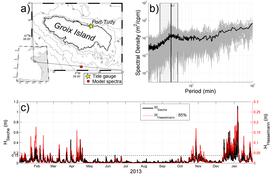
Figure 14: a) Location and bathymetric map of Groix Island and Port-Tudy. b) Background spectra (grey lines) and mean background spectrum (black line) computed on time series (calm periods) recorded with Port-Tudy tide gauge. The grey box represents the range of eigen periods obtained with the model. c) Significant height of seiche ( H_{\text{Seiche}} ) and IG waves ( H_{\text{Hasselmann}} ) time-series during the whole year 2013 and the first month of 2014.
