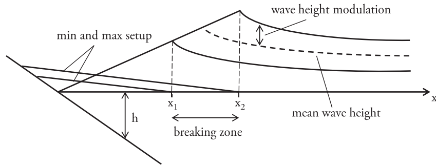
Figure 3: Schematic representation of the cross-shore variation of the minimum, mean and maximum short wave height, with the associated steady state setup through the surf zone. x_1 and x_2 are the minimum and maximum positions of the breakpoint, and h is the water depth. (Figure reproduced from Symonds et al. (1982).)
