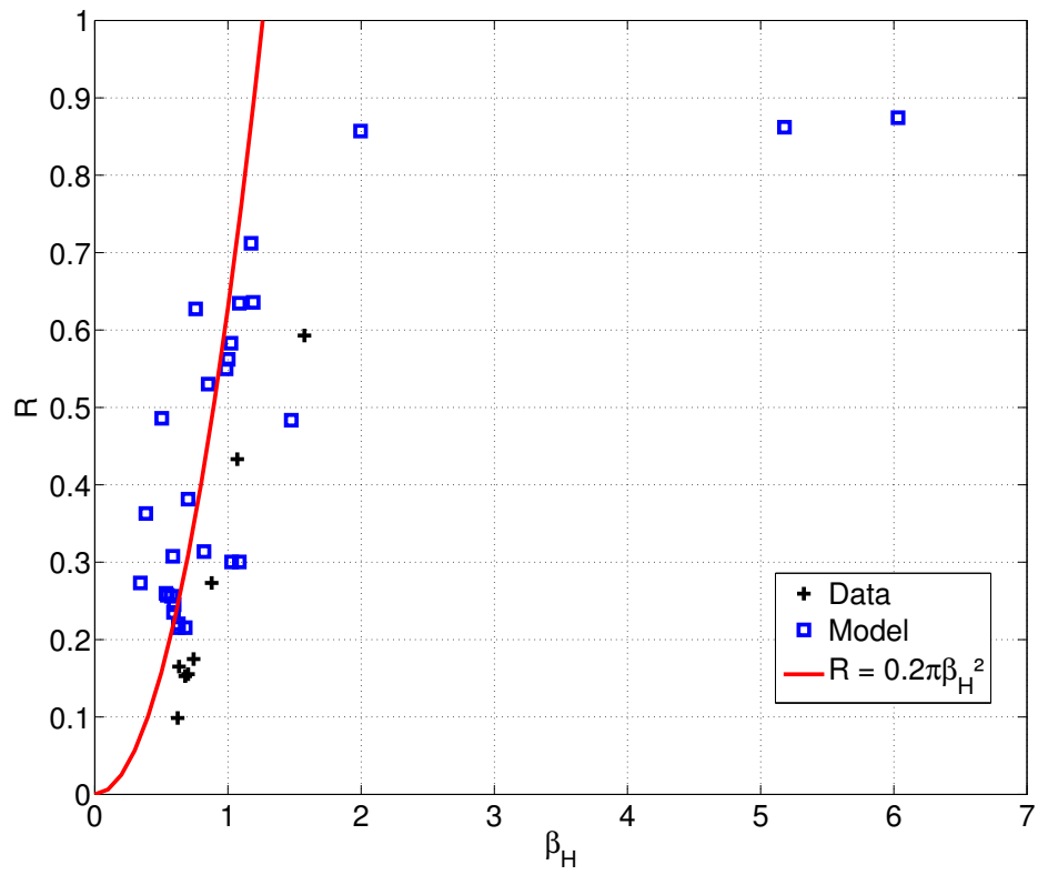
Figure 6: Relations between the reflection coefficient R and the normalized bed slope parameter \beta_H , modified from Van Dongeren et al. (2007)
