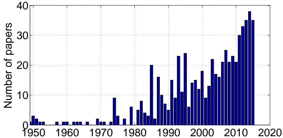
Figure 1: Number of paper per year found in Scopus and Web of Science where the title includes infragravity waves or surf-beat.
