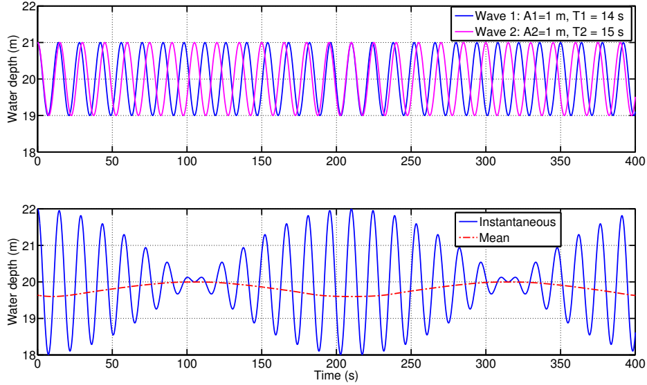
Figure 2: (A) Time series of two sinusoidal waves with periods of 14 s (blue) and 15 s (pink) travelling over a flat bottom by 20 m water depth. (B) Resulting free surface elevation (blue) and bound wave (red) as computed according to Longuet-Higgins and Stewart (1962).
