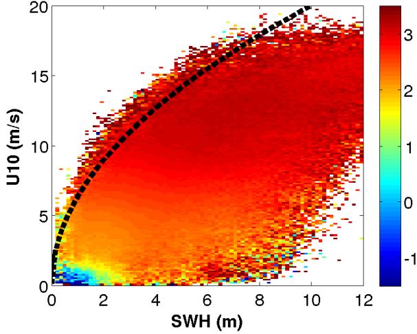
Fig. 4: Difference (in dB) between the Ku- and Ka-band mean NRCS. The Pierson-Moskowitz relationship SWH = 0.025 U_{10}^2 for fully developed seas is shown in dashed black lines and limits the available SWH - U_{10} domain.
