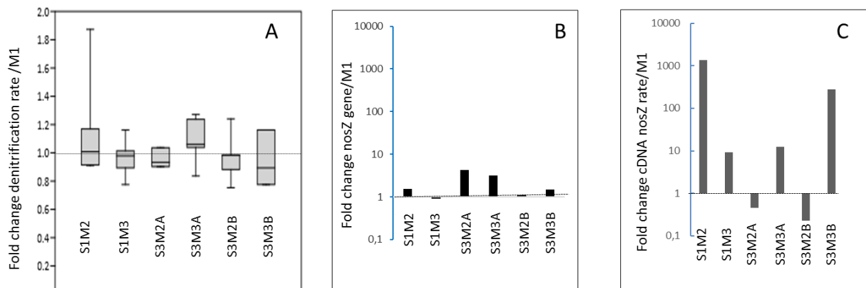
Fig. 4. Potential denitrification rate (A), abundance of denitrifiers ( nosZ gene)(B), nosZ induction rate (mRNA nosZ ) (C) at the end of the phase 3 expressed as fold change compared to control microcosms. (A) Results are presented as box-plots: the center vertical line marks the median, the edges of the box mark first and third quartiles and the vertical lines indicate the range of values that fall within 1.5 (midrange) of the hinges, (B) ratio of DNA- nosZ /DNA-16S rRNA normalized with control ratio, (C) Induction rate correspond to ratio of cDNA- nosZ /cDNA-16S rRNA normalized with control ratio. Ratio of 1 was marked with an horizontal hatched bar.
