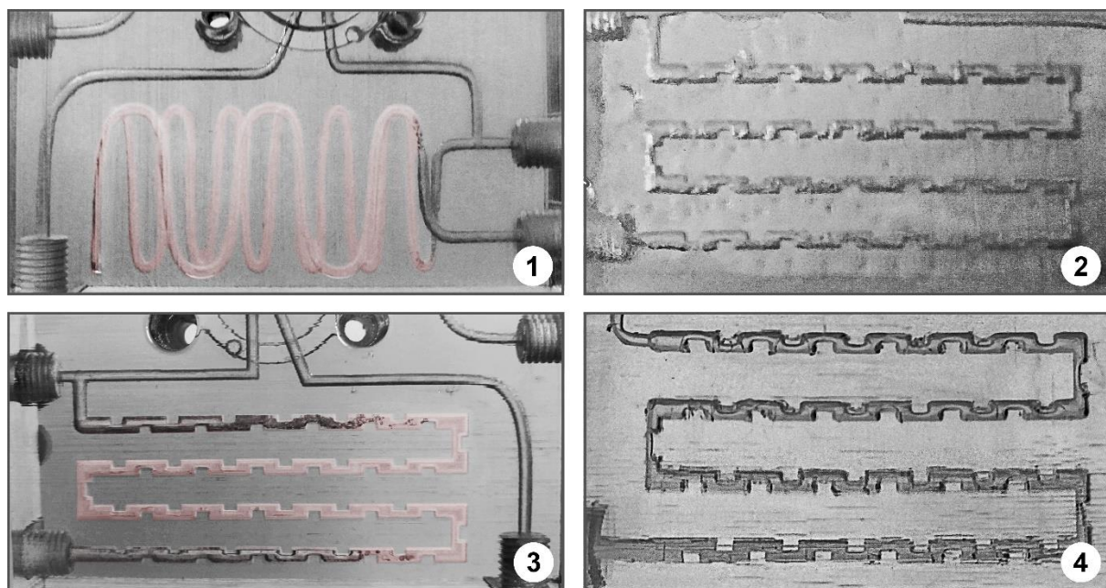
7 Figure 2. Mixing coils printed with different technologies: Polyjet (1;3), Stereolithography 8 (2), DLP (4).
