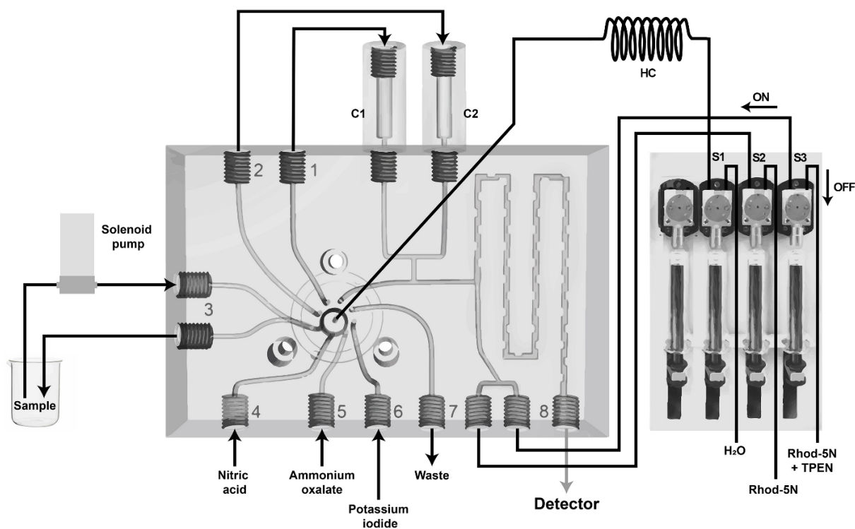
3 Figure 1. MSFIA-LOV system used for cadmium and lead determination with C1 column for 4 lead extraction and C2 column for cadmium.
