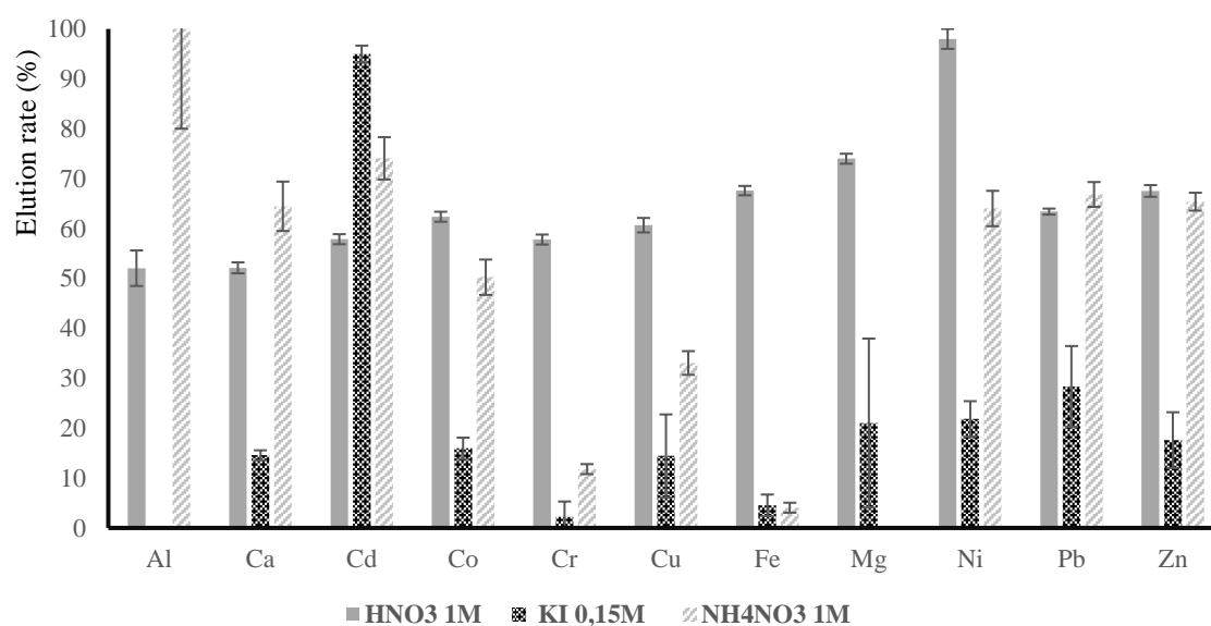
2 Figure 2. Elution rate of a multi-metal solution ( 10 \mu\text{mol.L}^{-1} for each metal) on Amberlite® IR 3 120 H with different eluents.
