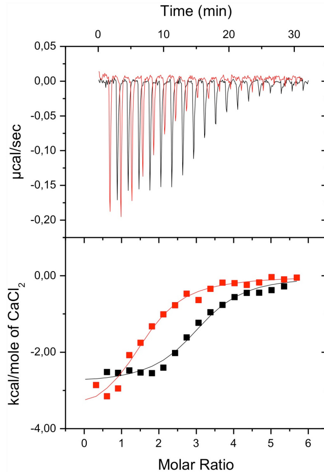
Fig 2. Typical ITC curves (upper panel) and binding isotherms (lower panel) of NOX5-EF interaction with CaCl 2 with (red line) or without (black line) incubation with 50 mM H 2 O 2 in 50mM Tris buffer (pH 7.5). All ITC titrations were performed in triplicate.
