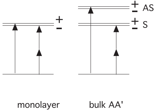
FIG. 4. Allowed transitions towards the lowest excitonic states with circularly polarized light. (Left) Monolayer; the \Phi^+ ( \Phi^- ) is excited with a one-photon (two-photon) process, where \Phi^\pm denote the two circularly components of the degenerate 1s exciton. (Right) Bulk AA' stacking; there are now two antisymmetric (AS, odd, one-photon allowed) and symmetric (S, even, two-photon allowed) degenerate states, separated by a Davydov splitting.
