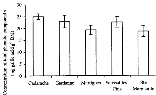
Fig. 2. Mean concentrations of total phenolic compounds in needles of Aleppo pine ( \text{mg gallic acid g}^{-1} dry matter \pm standard deviation) for the various study sites.
