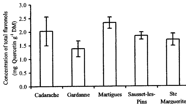
Fig. 4. Mean concentrations of total flavonols in needles of Aleppo pine ( \text{mg of quercetin g}^{-1} dry matter \pm standard deviation) for the various study sites.
