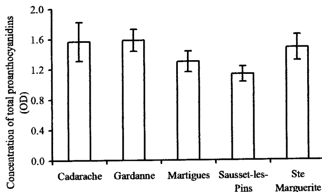
Fig. 3. Concentrations of total proanthocyanidins in needles of Aleppo pine (optical density [OD] \pm standard deviation) for the various study sites.
