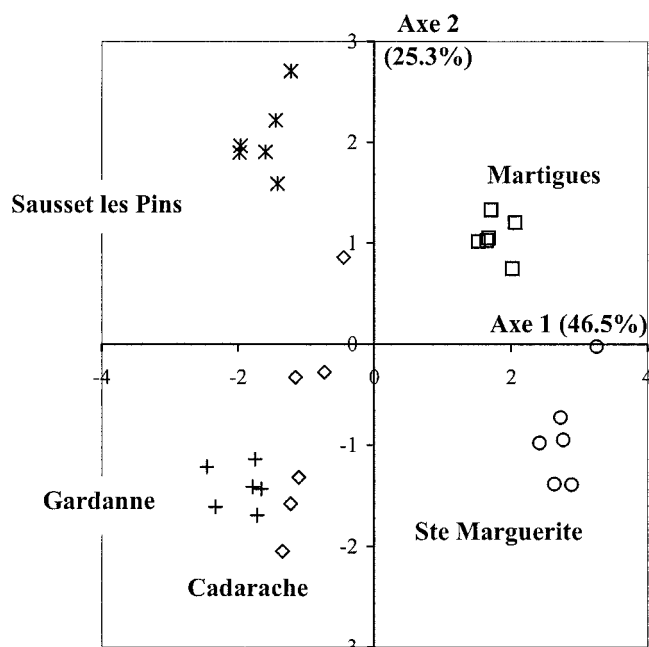
Fig. 5. Two-dimensional mapping of the principal component analysis performed for total phenols, total proanthocyanidins, total flavonols, and air pollutants.
