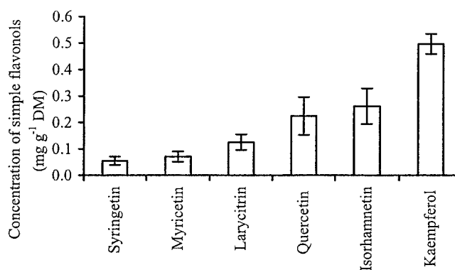
Fig. 6. Mean concentrations of simple flavonols (in mg g -1 dry matter ± standard deviation) for the whole set of study sites.
