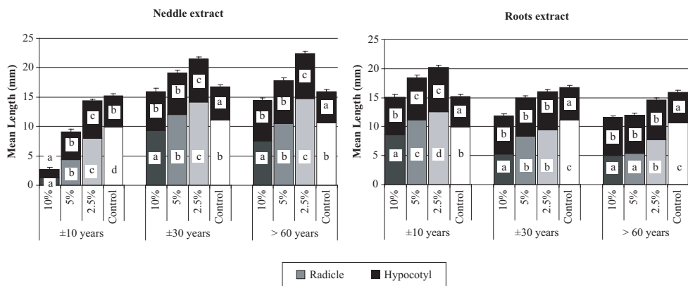
Fig. 4 Mean length of radicle and hypocotyl (and confidence interval at 95%) of L. strictum as a function of P. halepensis age, organ nature (root or needle), and extract dose. Tukey's tests with regard to dose effects are also presented for each organ (radicles in normal style and hypocotyls in italics). Value not different at \alpha = 5\% are denoted with the same letter
