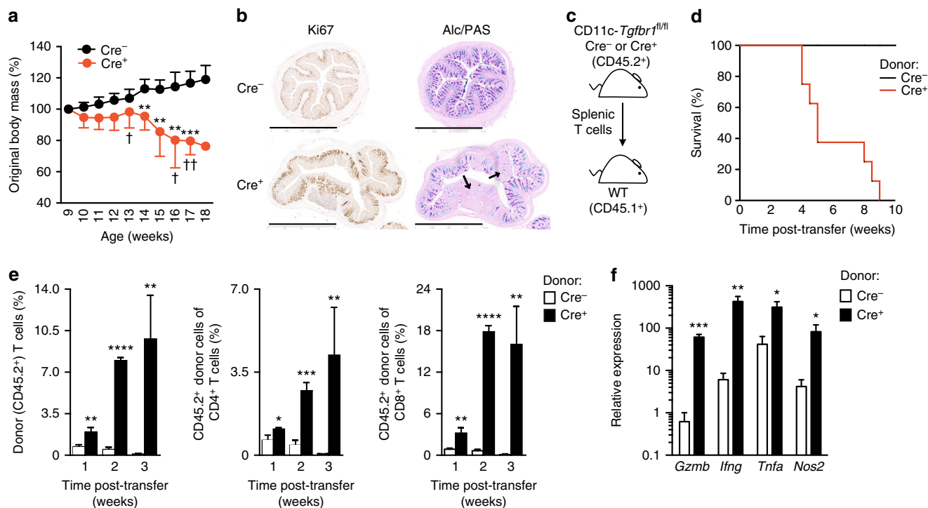
Fig. 1 T-cell-dependent inflammatory disease in CD11c-Cre. Tgfb1 fl/fl mice. a Body weights of CD11c-Cre. Tgfb1 fl/fl ( Cre + ) mice and Tgfb1 fl/fl ( Cre - ) mice littermate controls presented as a percentage of original bodyweight at 9 weeks of age. The results are the means \pm 1 SD of five ( Cre + ) or six ( Cre - ) mice per group and are representative of two experiments (** p < 0.01 and *** p < 0.001—Student's t -test followed by Holm-Sidak correction). († indicates the loss of animal from group). b Representative colonic pathology as assessed by epithelial cell turnover (Ki67 staining—left panels) and goblet cell density (PAS staining—right panels) in Cre - (upper panels) and Cre + mice (lower panels). Arrows indicate loss of goblet cells. Scale bar, 1 mm. c Experimental scheme for the transfer of splenic T cells from Cre - or Cre + mice into congenic WT recipients. d Survival of WT recipients given T cells from Cre - or Cre + mice. Data are pooled from two experiments with a total of seven ( Cre - ) or eight ( Cre + ) mice per group. e Frequency of CD45.2 + donor T cells among total blood T cells (left) and the frequency of donor cells within the CD4 + and CD8 + T-cell compartments (centre and right) at 1, 2 and 3 weeks post transfer in the mice from c , d above. Data are from one of two independent experiments each with 3 ( Cre + ) or 4 ( Cre - ) mice per group. f Expression of mRNA transcripts for Gzmb , Ifng , Tnfa and Nos2 in the stomach of recipients of splenic T cells from Cre - or Cre + mice in d above. In e , f , bars represent the mean \pm SD of three mice per group and mRNA expression is relative to expression of Gapdh . * p < 0.05, ** p < 0.01, *** p < 0.001 and **** p < 0.0005 determined by two-tailed Student's t -test
