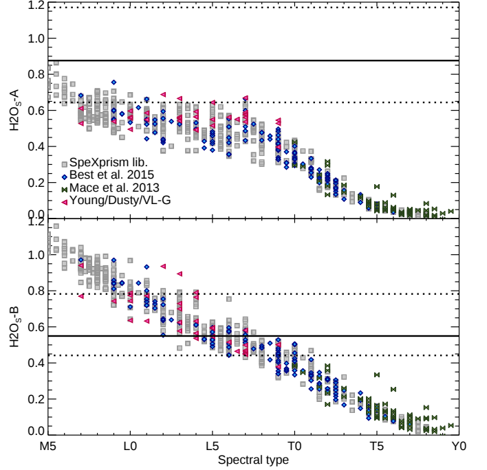
Fig. 10. Evolution of the spectral indices H_{2O_S-A} and H_{2O_S-B} . We overlaid the value of the indices (thick line) and the associated error (dotted line) computed on the HD 206893b spectrum.
