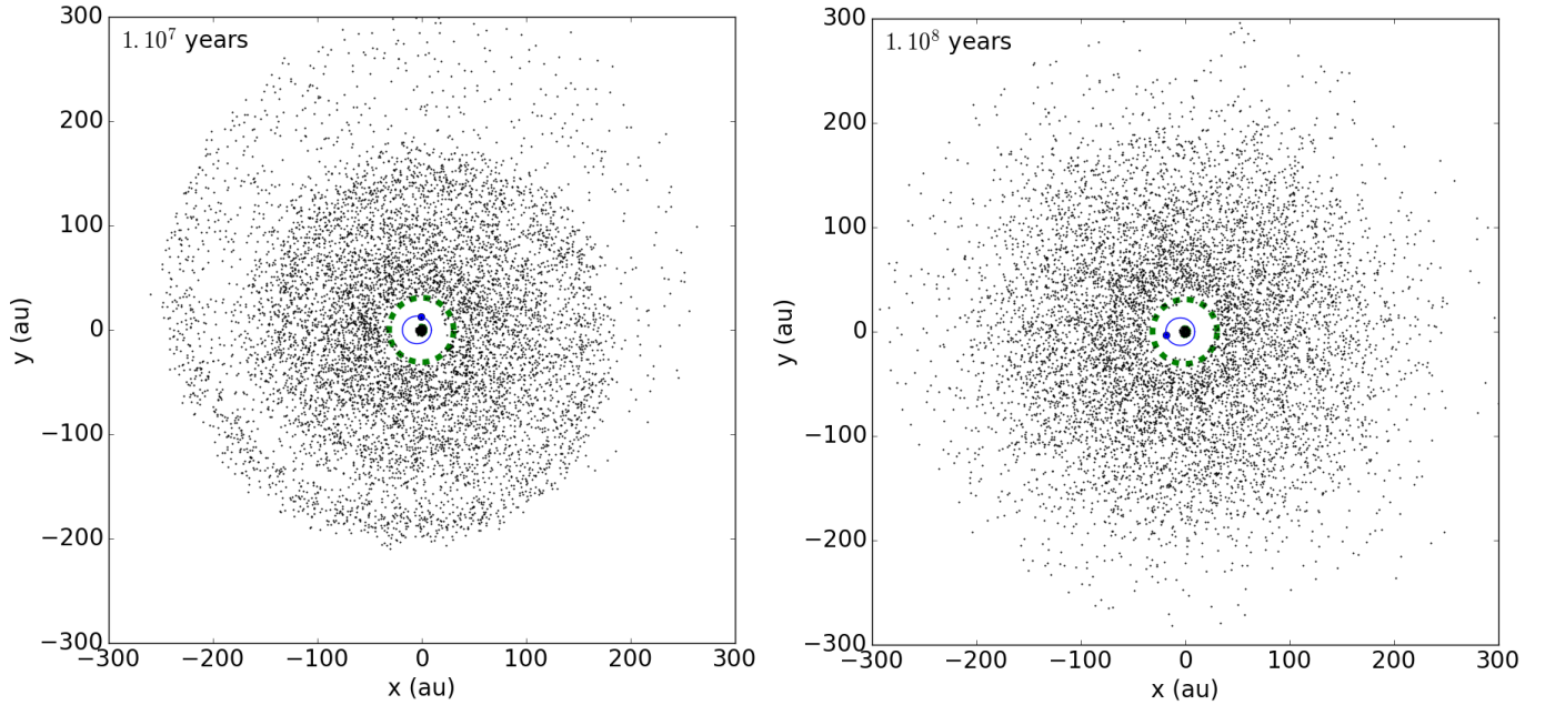
Fig. 22. Representation of an N -body simulation of 10 000 test particles initially ranging from 1 to 200 AU after a ) 10 million years; b ) 100 million years. A companion has been injected at t = 0 with semi-major axis 14.2 AU and eccentricity 0.31. Its orbit is depicted in blue, while the gap outer extent given by Eq. (4) is in green.
