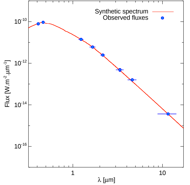
Fig. 6. BT-NEXTGEN synthetic spectrum (red curve) adjusted onto the star photometry (blue dots).
