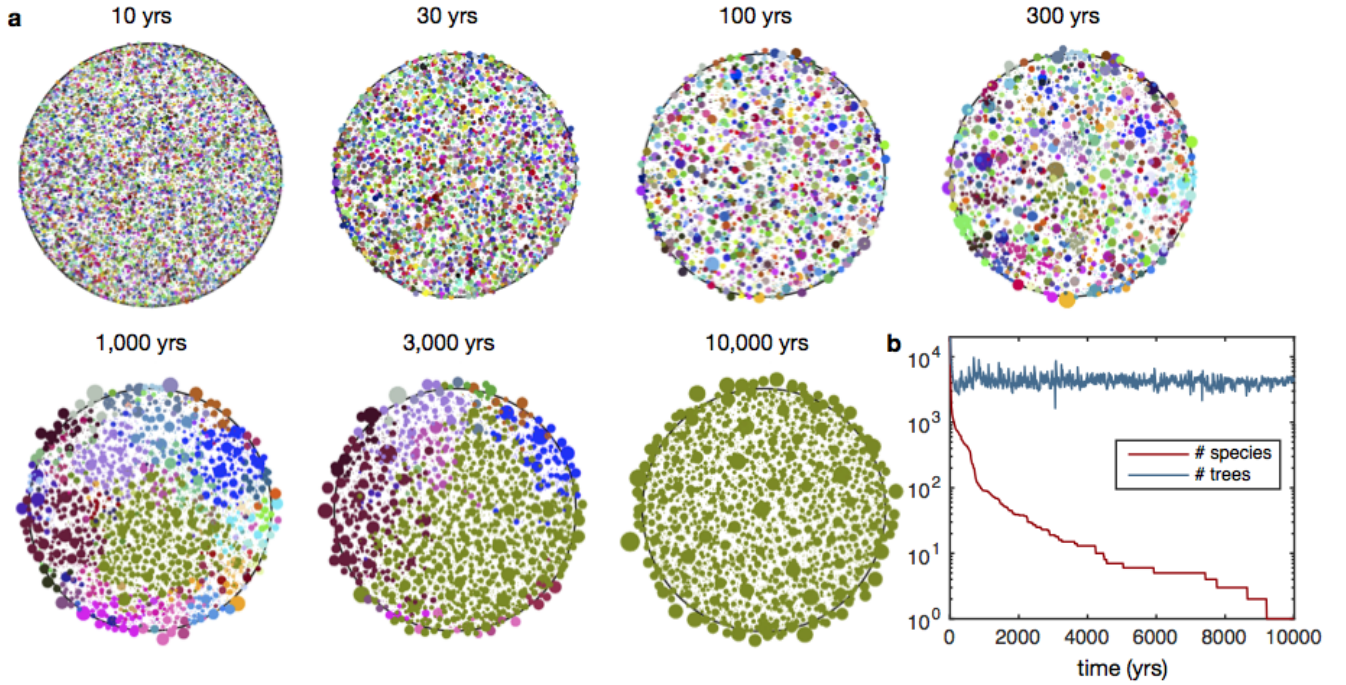
Figure 2. Evolution of a forest on a virtual island. (a) Example of the evolution of a virtual forest over 10,000 yrs (see Supplementary Movie 1). Initially, 20,000 trees with random genomes are sown. Each circle is a tree whose centre is at the centre of gravity of foliage, and whose radius is the standard deviation of the foliage distribution projected onto the ground. The outer black circle of radius R = 200L is the habitat limit. Colours are determined using three neutral marker genes as RGB values. Because trees growing at the periphery are on average larger than the others, allometric statistics (see below) are performed on trees with their trunk in a central zone of radius 0.9R . (b) Number of trees and number of species as a function of time, for the same forest as in (a).
