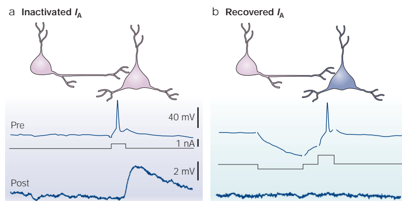
Figure 7 | Gating of action-potential propagation by the potassium current I_A .
