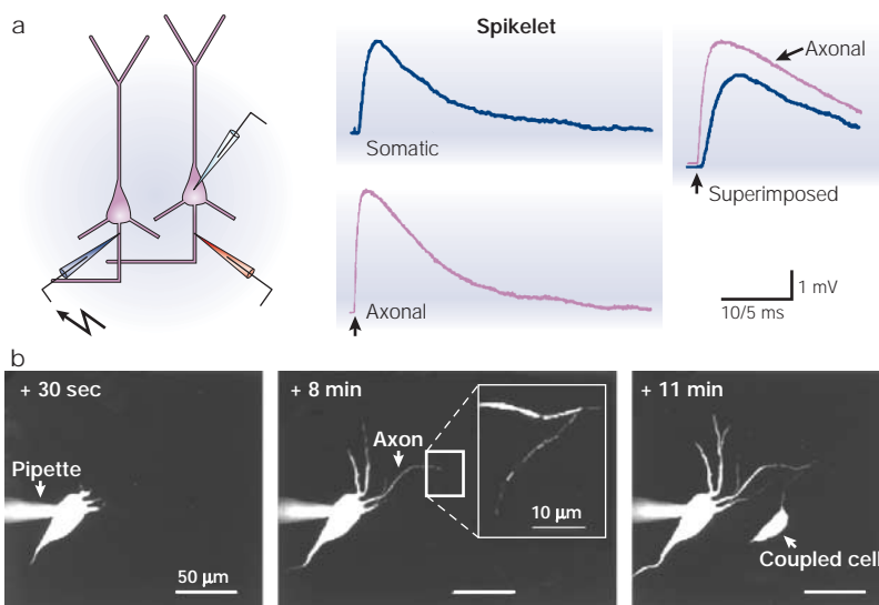
Figure 9 | Axo-axonic coupling of hippocampal pyramidal neurons. a | Spikelets propagate antidromically. Whole-cell recordings were obtained from the soma (blue traces) and from the axon hillock (pink traces). Spikelets were evoked by the stimulation of the axon of a neighbouring neuron. Superimposed traces show a delay between the axonal recording and the somatic recording, indicating that spikelets traverse the axon prior to invading the soma. b | Dye coupling between hippocampal pyramidal neurons. A neuron was recorded in whole-cell configuration with a pipette containing a fluorescent dye (+ 30 sec). Axon and dendrites were labelled about 8 min after establishing whole-cell configuration. The boxed region shows an axon of a second pyramidal neuron containing dye from the axon of the first cell. The cell body of the dye-coupled pyramidal cell appears a few minutes later (+ 11 min). Adapted, with permission, from REF. 119 © (2001) Cell Press.
