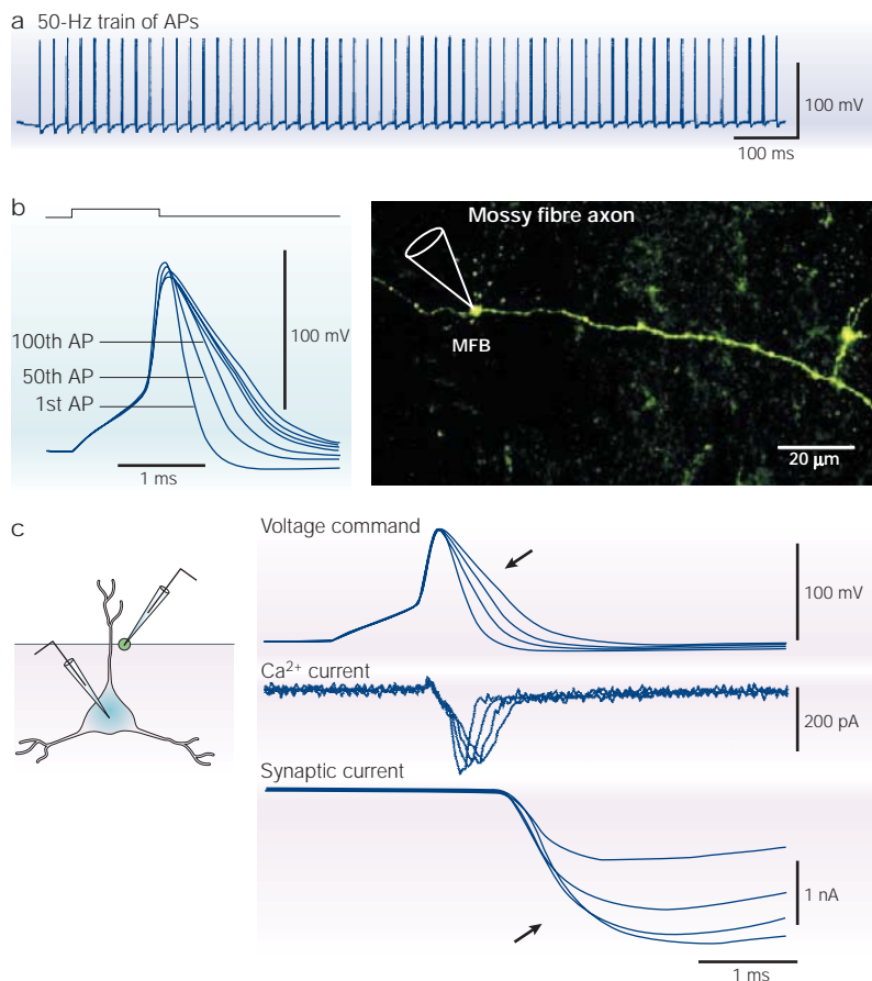
Figure 1 | Shaping of the action potential in the axon. a | A mossy fibre bouton (MFB) is recorded in the whole-cell configuration and activated at a frequency of 50 Hz. b | During repetitive stimulation of the axon, the action potential (AP) becomes wider. Every fiftieth AP is compared with the first AP in the train. c | AP broadening potentiates transmitter release. The mossy fibre terminal (green) and the corresponding CA3 cell (blue) were recorded simultaneously. AP waveforms were imposed at the presynaptic terminal. The increased duration of the waveform incremented the presynaptic calcium current and potentiated the amplitude of the synaptic current. Adapted, with permission, from REF. 31 © (2000) Cell Press.
