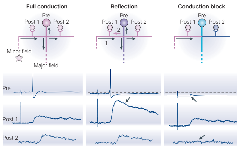
Figure 8 | Reflection of action potentials. Reflection and conduction block produce multilevel synaptic transmission in mechanosensory neurons of the leech. Left, an action potential that is initiated by anterior minor field stimulation invades the whole axonal arborization (pink) and evokes an excitatory postsynaptic potential in all postsynaptic cells. Middle, following repetitive stimulation, the cell body is slightly hyperpolarized (purple) and the same stimulation induces a reflected action potential at the branch point between the left branch and the principal axon. The reflected action potential (pink arrow 2) stimulates the presynaptic terminal on postsynaptic cell 1 twice, thereby enhancing synaptic transmission (arrow in lower panel). Right, when the cell body is further hyperpolarized (turquoise), the stimulation of the minor field now produces an action potential that fails to propagate at the branch point. The failed spike is seen as a spikelet at the cell body (upward arrow). No postsynaptic response is evoked in postsynaptic cell 2 (downward arrow). Adapted, with permission, from REF. 75 © (1998) The National Academy of Sciences.
