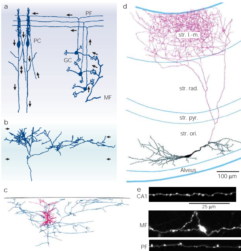
Figure 3 | Branch points and varicosities. a | Drawing of the cerebellar afferent circuit. Mossy fibre (MF) activity excites granule cells (GC) whose axons project towards the surface of the cortex. The GC axon bifurcates into two branches, which form the parallel fibres (PFs). Adapted from REF. 1. b | Reconstruction of the terminal bouquet of a thalamocortical axon in area 17 of the cat. Horizontal arrowheads indicate the limits of layer IV. Adapted, with permission, from REF. 44 © (1998) Society for Neuroscience. c | Dendritic (red) and axonal (blue) arborizations of a layer II pyramidal neuron in the barrel cortex. Adapted, with permission, from REF. 45 © (2003) Society for Neuroscience. d | Camera lucida reconstruction of a hippocampal GABA ( \gamma -aminobutyric acid)-containing interneuron. The dendritic arbor is represented in black and the dense axonal arborization in red. Adapted, with permission, from REF. 41 © (2000) American Association for the Advancement of Science. Str. l.-m.; stratum lacunosum-moleculare; str. ori.; stratum oriens; str. pyr.; stratum pyramidale; str. rad.; stratum radiatum. e | Varicosities on stratum oriens axons in the CA1 area (upper), on MF axons in area CA3 (middle) and on cerebellar PFs (bottom). Adapted, with permission, from REF. 53 © (2002) The National Academy of Sciences.
