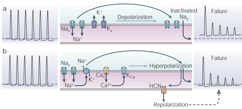
Figure 6 | Mechanisms of propagation failures induced by repetitive stimulation.
