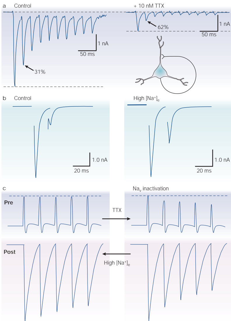
Figure 2 | The role of sodium channel inactivation in short-term synaptic depression. a | Repetitive stimulation of an autaptic contact produces short-term depression. The application of a low concentration of the channel blocker tetrodotoxin (TTX) reduces synaptic transmission and enhances short-term depression. Adapted, with permission, from REF. 36 © (2000) Society for Neuroscience. b | Rescue of paired-pulse transmission by elevation of the extracellular sodium concentration ( [Na^+]_e ). The large paired-pulse depression that is observed at an autaptic contact of a cultured hippocampal cell is dramatically reduced when [Na^+]_e is increased by 40 mM. Adapted, with permission, from REF. 38 © (2002) The American Physiological Society. c | Hypothetical regulation of short-term depression by the modulation of activity-dependent attenuation of presynaptic spike amplitude. Sodium channel inactivation (TTX, right column) attenuates the spike train and enhances depression. Reduced inactivation (high [Na^+]_e , left column) opposes both presynaptic spike attenuation and short-term depression.
