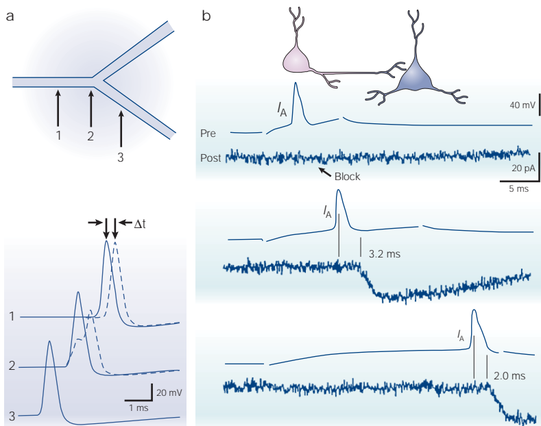
Figure 4 | Axonal propagation and spike timing. a | Comparison of the delay of propagation introduced by a branch point with a geometrical ratio (GR) > 1 (dashed traces) versus a branch point with perfect impedance matching (GR = 1, continuous traces). Upper, schematic drawing of a branched axon with three points of recording. At the branch point with GR = 8, the shape of the action potential is distorted and the propagation displays a small latency ( \Delta t ). Adapted, with permission, from REF. 62 © (1991) The Biophysical Society. b | Propagation failures in hippocampal cell axons are associated with conduction delays. The presynaptic neuron (Pre) was slightly hyperpolarized with constant current to remove inactivation of the A-current. A presynaptic action potential induced with a short delay after onset of the depolarizing pulse did not elicit excitatory postsynaptic current in the postsynaptic cell (Post) because of the large activation of I_A . Increasing the delay permitted action potential propagation because I_A was reduced during the action potential. For complete inactivation of I_A (lower pair of traces), latency decreased. Adapted, with permission, from REF. 66 © (1997) Macmillan Magazines Ltd.
