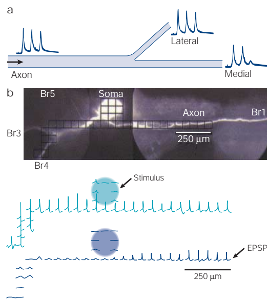
Figure 5 | Propagation failures. a | Propagation failure at a branch point in a lobster axon 33 . b | Propagation failure at the junction between an axonal branch and the soma of a snail neuron (metacerebral cell). The propagation in the axonal arborization was analysed by the local fluorescence transients owing to the action potential. The recording region is indicated by an outline of a subset of individual detectors, superimposed over the fluorescence image of the neuron in situ . When the action potential was evoked by direct stimulation of the soma, it propagated actively in all axonal branches (green traces). By contrast, when the action potential was evoked by the synaptic stimulation (EPSP) of the right axonal branch (Br1), the amplitude of the fluorescent transient declined when approaching the cell body, indicating a propagation failure (blue traces). Adapted, with permission, from REF. 87 © (2000) The Physiological Society.
