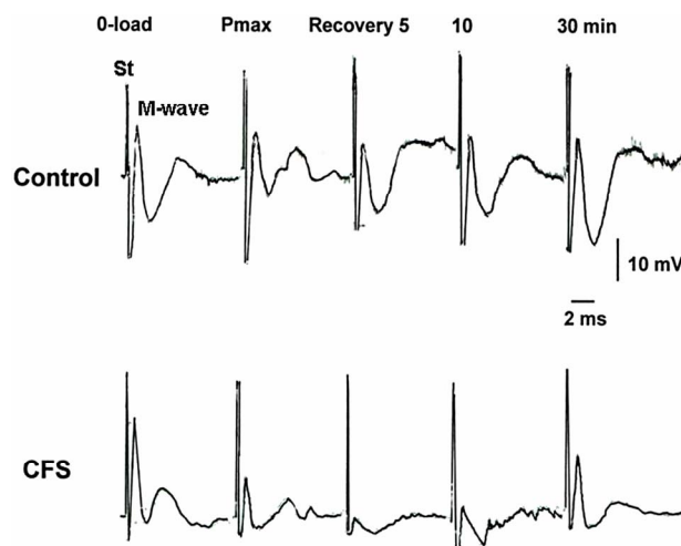
Figure 2. Examples of M-wave recordings in vastus lateralis muscle in a control (healthy) subject and a CFS patient in the I group at rest, VO 2 max, and during the 30-min post-exercise recovery period. Stimulus (St) and M-wave are indicated.
