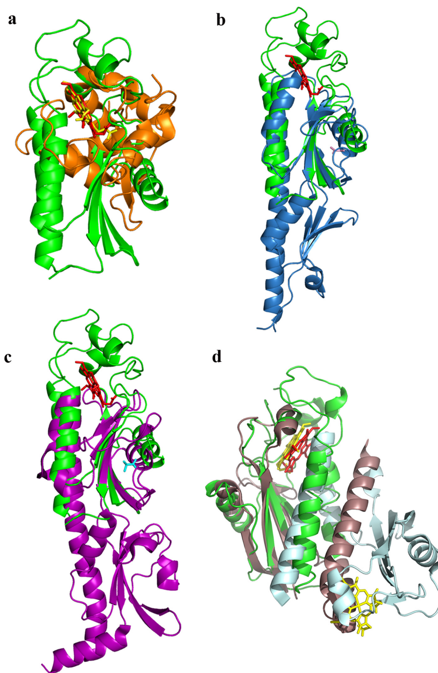
Figure 6. Structural comparison of the Tll0287 protein with other proteins. a , superposition of Tll0287 and PsbV2 from T. elongatus (PDB code 4LJI) (37). The colors for the Tll0287 protein and its heme are green and red , respectively, and those for the PsbV2 protein are as follows: heme, yellow ; others, orange . b , superposition of Tll0287 and the sporulation kinase D sensor domain from B. subtilis ( blue , A chain of PDB code 4JGO; pink , the ligand of this protein, pyruvate) (48). c , superimposition of Tll0287 and a methyl-accepting chemotaxis protein (Mcp) ( purple , A chain of PDB code 3C8C; cyan , the ligand of this protein, alanine). d , superimposition of Tll0287 and the dimer of the non-membrane part of GSU0935 (PDB code 3B42) (62).
