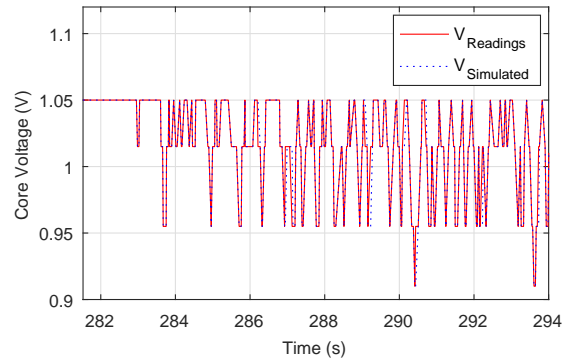
Figure 9: Voltage model estimations vs system readings.
