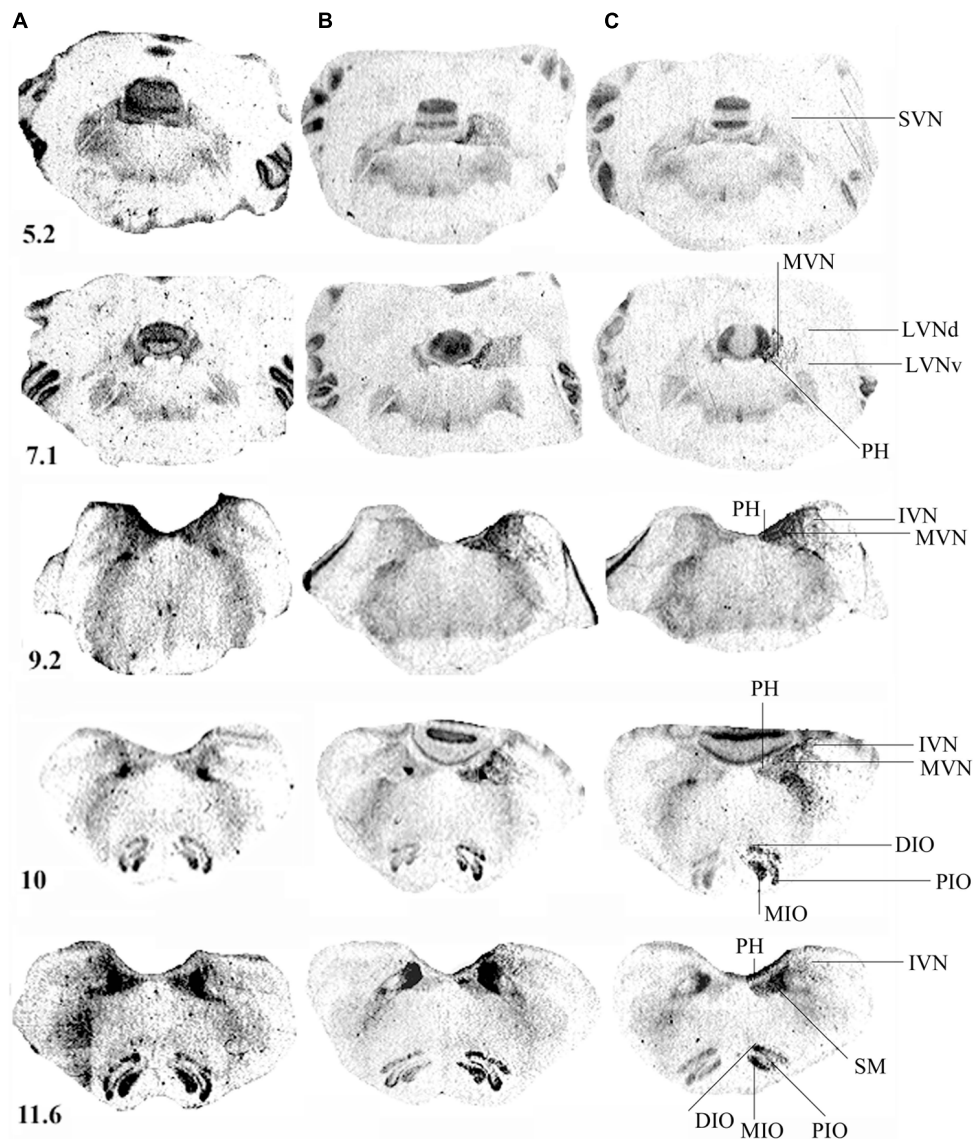
FIGURE 3 | (A–C) [ ^3\text{H} ]N- \alpha -methylhistamine binding sites in the cat brainstem. Coronal sections from three representative control and unilateral vestibular neurectomized cats showing decreases in histamine \text{H}_3 receptor binding in the different structures of the brainstem on the lesioned side (left side in the figure) 1 (B) or 3 (C) weeks after unilateral vestibular neurectomy, as compared to the controls (A). Illustrations are given for serial sections
