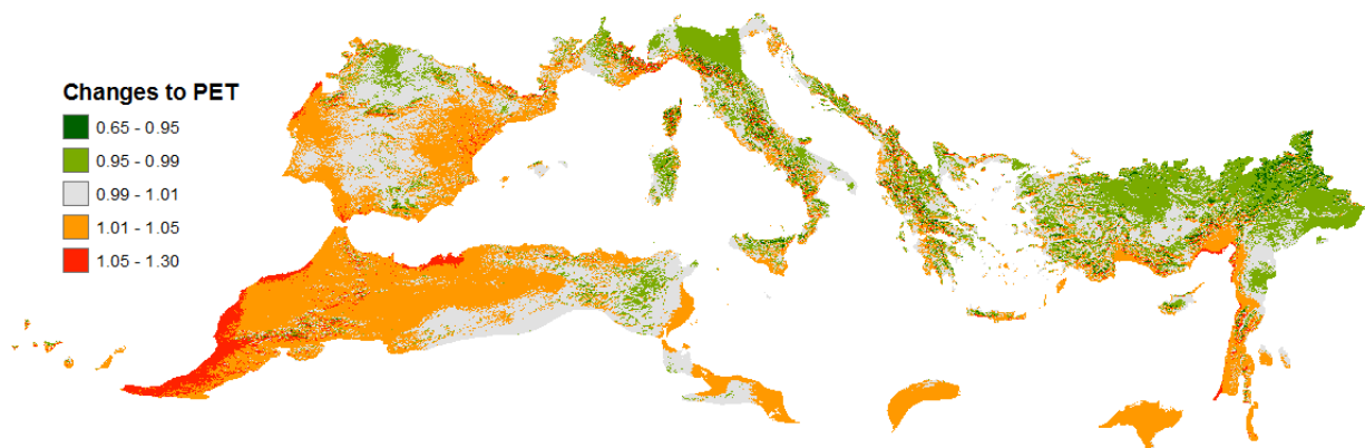
Fig. H.1 Changes in annual PET until 2050 based on the 19 CMIP5 simulations of the RCP4.5 for the Mediterranean ecoregion. The future decrease in the temperature range is balancing the increase in the mean temperature, leading to a decrease in PET in some areas (marked as green on the figure).
