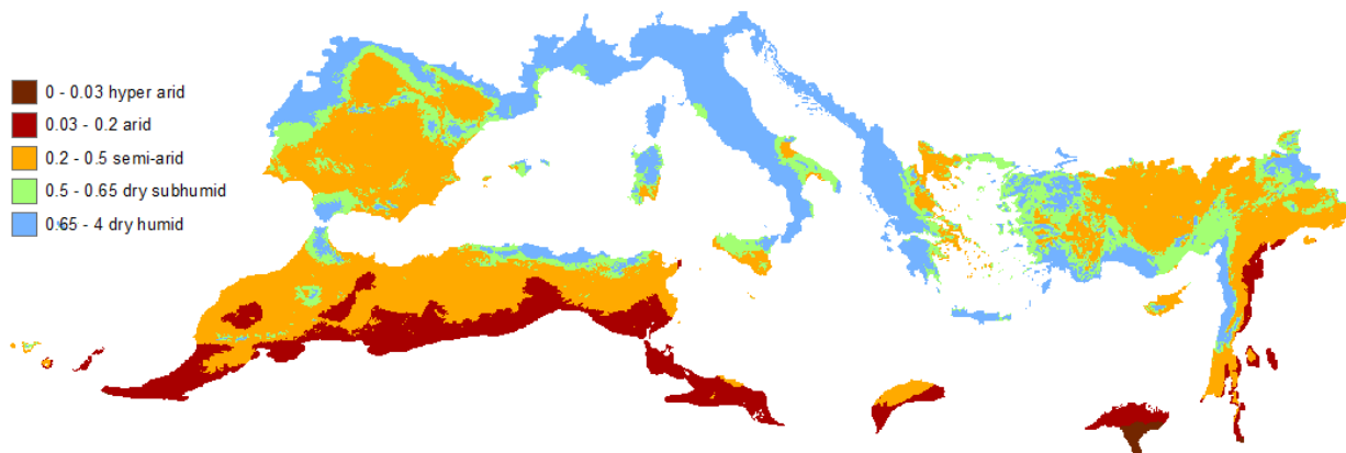
Fig. H.2 Current aridity index (Zomer et al. 2008)
