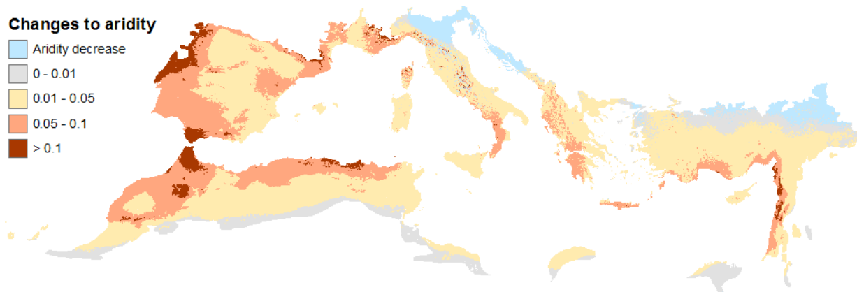
Fig. H.3 Changes to aridity until 2050 based on the 19 CMIP5 simulations of the RCP4.5 for the Mediterranean ecoregion
