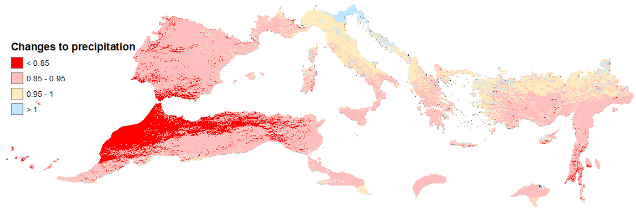
Fig. G.1 Changes in precipitation until 2050 (compared to current climate, represented by the 1960-1990 average) based on the mean of 19 CMIP5 simulations of the RCP4.5 for the Mediterranean ecoregion
