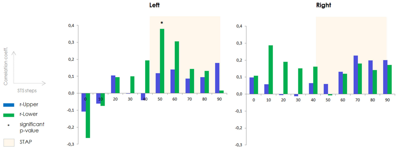
Fig. 4 Linear correlation (Pearson) between STS depth and functional activity along ten steps on the STS. The first coordinate of each step is indicated below the corresponding bar. Bars represent the correlation coefficients ( r ) obtained from the upper ( blue ) and lower
