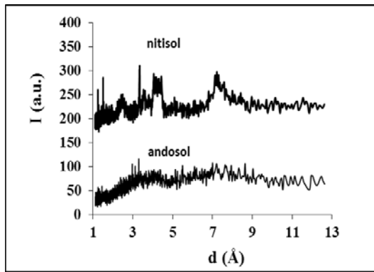
Figure1: X-rays typical diffractogram of volcanic soils samples. Counts versus lattice spacing d (Å)
