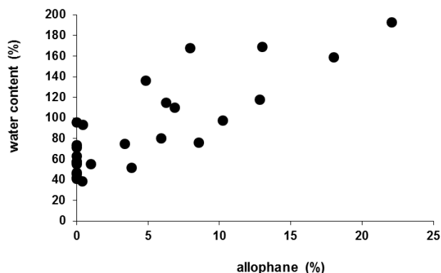
Figure7: Water content in volcanic soils versus allophane content
