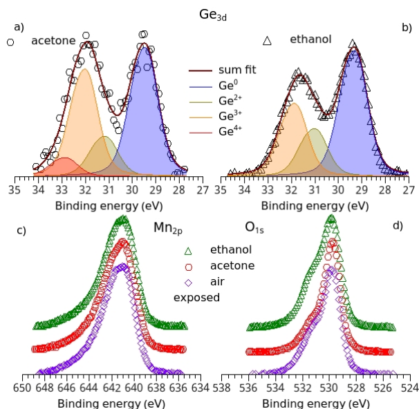
Figure 2: XPS analysis of the \text{Mn}_5\text{Ge}_3 surface after exposure to acetone and ethanol. a) and b) \text{Ge}_{3d} core level. c) \text{Mn}_{2p_{3/2}} and d) \text{O}_{1s} core levels. (For c) and d), the air exposed case is included as a comparison).
